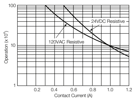
Electrical endurance
