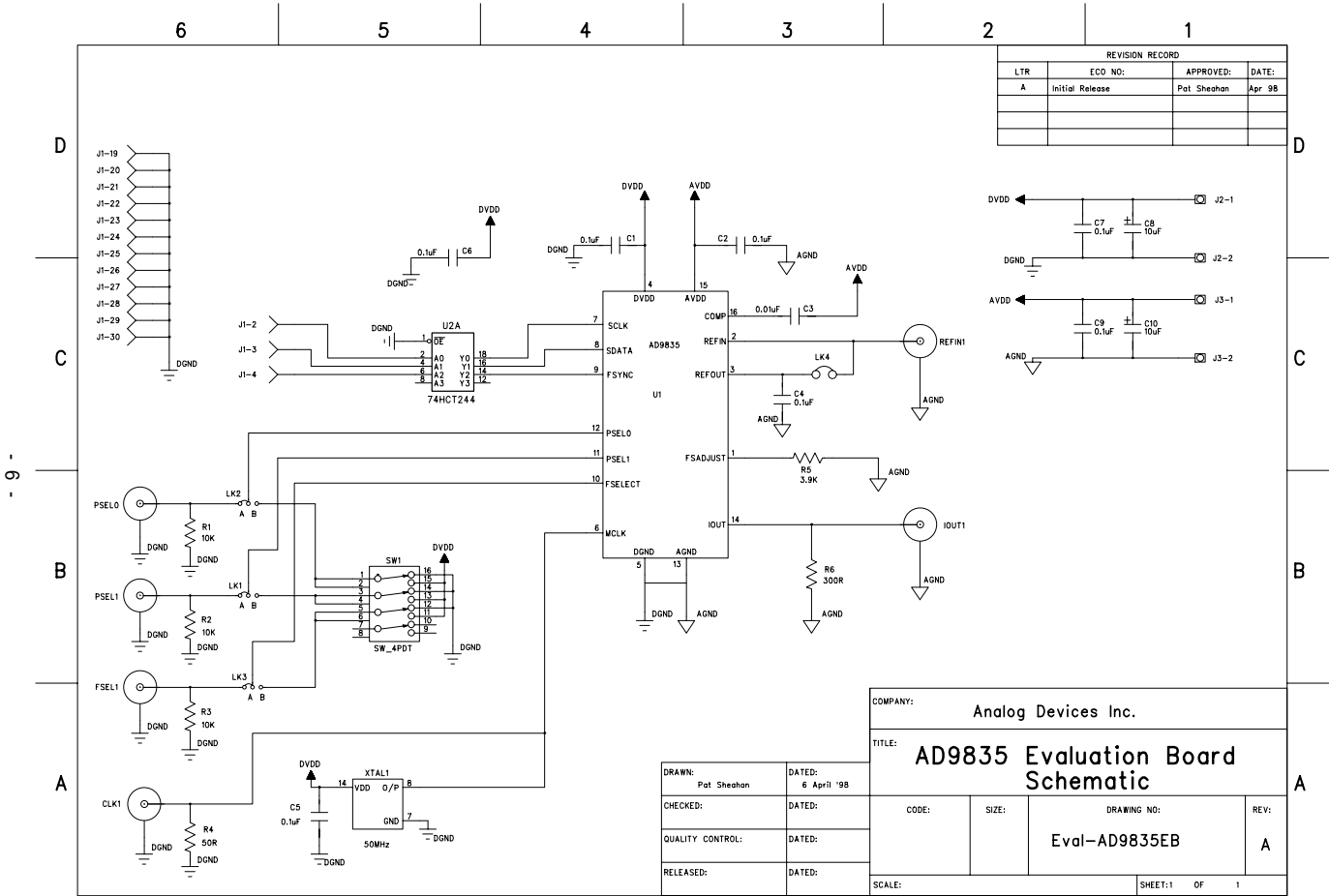
Figure 4: Eval-AD9835EB Schematic
