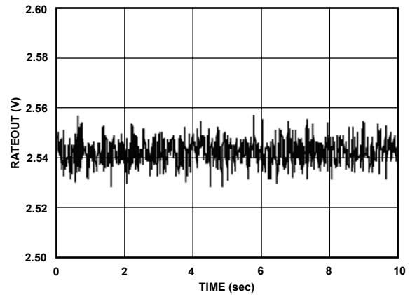
Figure 25. Random Vibration (Lateral) 2 Hz to 40 Hz, 3.2 g rms
