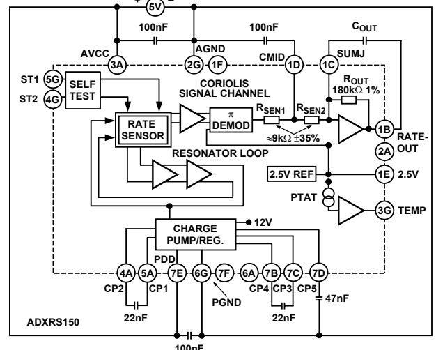
Figure 23. Block Diagram with External Components
