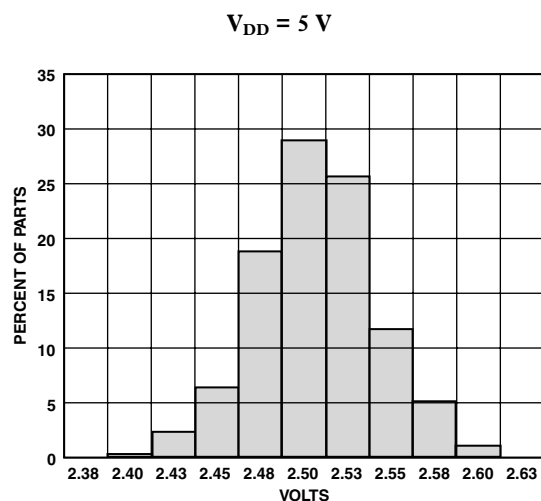
TPC 4. X-Axis Zero g Bias Distribution at X_{FILT} , V_{DD} = 5\text{ V}
