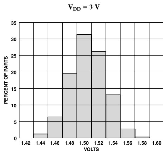
TPC 1. X-Axis Zero g Bias Distribution at X_{FILT} , V_{DD} = 3\text{ V}
