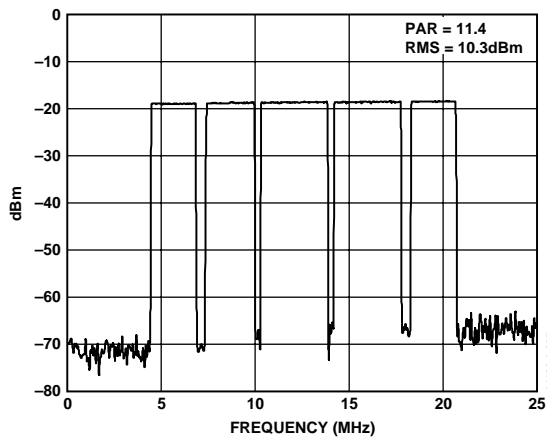
Figure 40. Spectral Plot of 84-Carrier OFDM Test Vector Using IAMPN in Current-Mode Configuration (IAMP Settings of I = 10 mA, N = 4 , G = 0 ; V_{CM} = 4.8 V)
