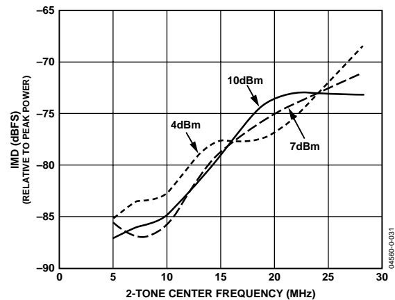
Figure 31. 2-Tone IMD Frequency Sweep vs. Peak Power with f_{DATA} = 80 MSPS, 2× Interpolation
