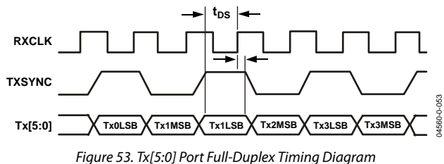
Figure 53. Tx[5:0] Port Full-Duplex Timing Diagram
