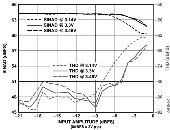
Figure 11. SINAD and THD vs. Input Amplitude and Supply ( f_{IN} = 8 MHz, LPF f_{-3dB} = 26 MHz; RxPGA = 0 dB)
