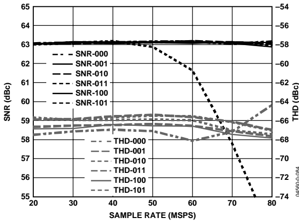
Figure 84. SNR and THD Performance vs. f_{ADC} and ADC Bias Setting with RxPGA = 0\text{ dB} , f_{IN} = 10\text{ MHz} , A_{IN} = -1\text{ dBFS}
