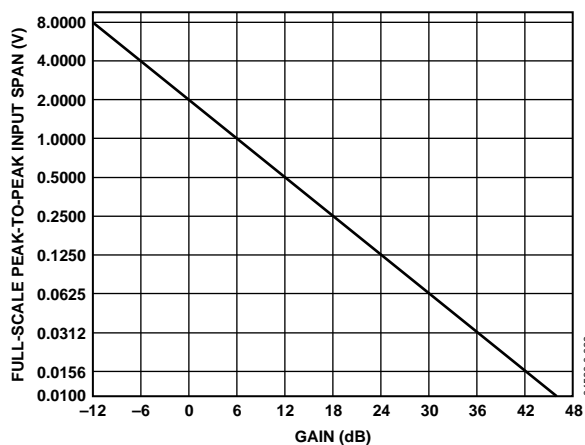
Figure 69. Maximum Peak-to-Peak Input vs. RxPGA Gain Setting that Does Not Result in ADC Clipping
