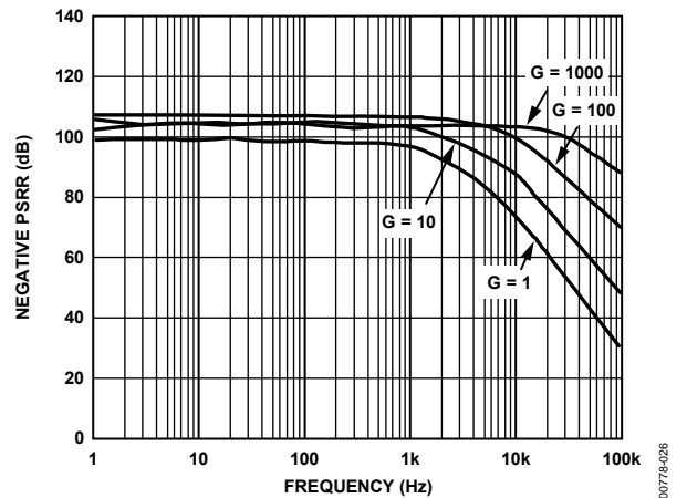
Figure 26. Negative PSRR vs. Frequency, \pm 5 \text{ V}_S
