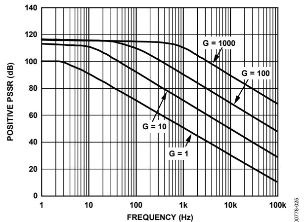
Figure 25. Positive PSRR vs. Frequency, 5 \text{ V}_S , 0 \text{ V}_S
