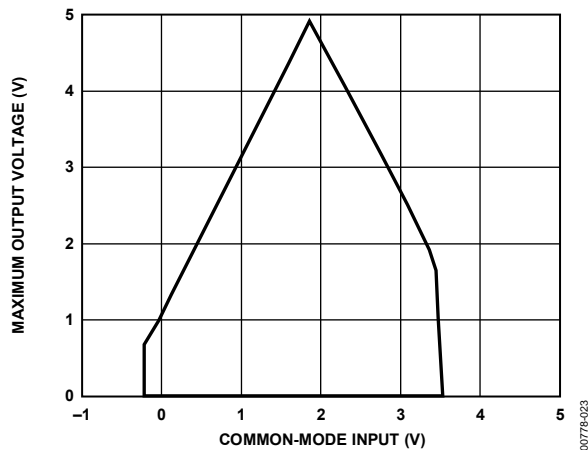
Figure 23. Maximum Output Voltage vs. Common-Mode Input, G \geq 10 , V_S = 5 \text{ V} , R_L = 100 \text{ k}\Omega
