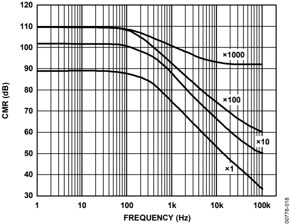
Figure 18. CMR vs. Frequency, \pm 5 V_S
