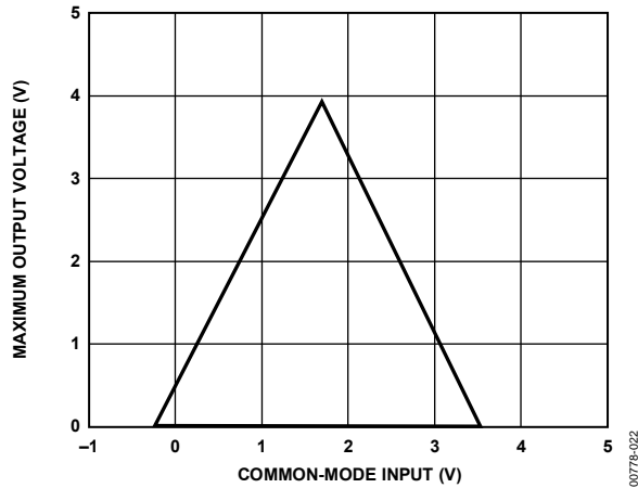
Figure 22. Maximum Output Voltage vs. Common-Mode Input, G = 1 , V_S = 5 \text{ V} , R_L = 100 \text{ k}\Omega
