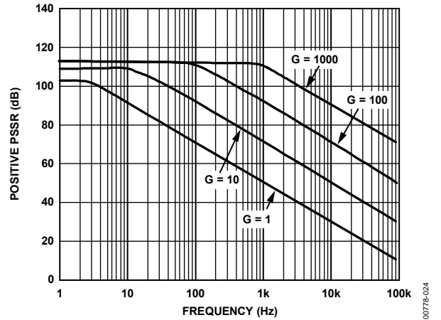
Figure 24. Positive PSRR vs. Frequency, \pm 5 \text{ V}_S
