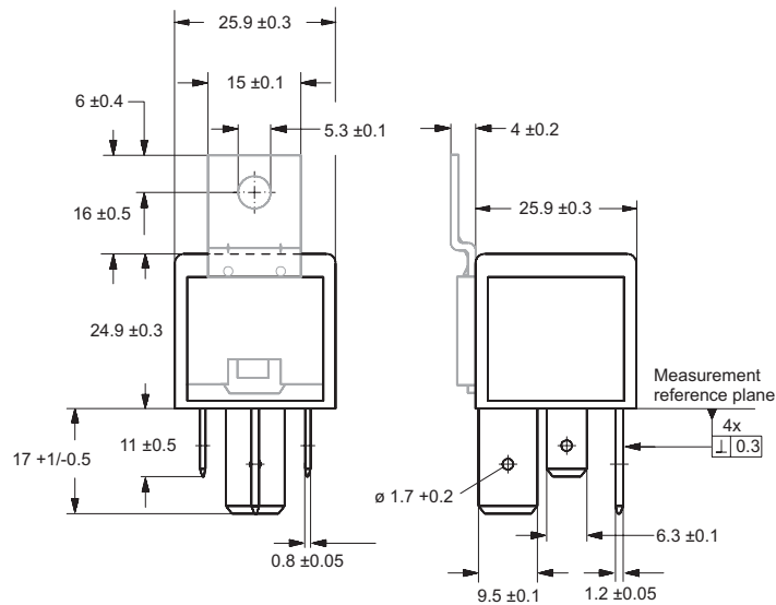
Quick connect terminal similar to ISO 8092-1
