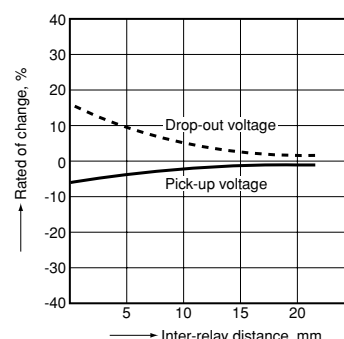
3. Influence of adjacent mounting
