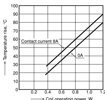
2. Coil temperature rise
