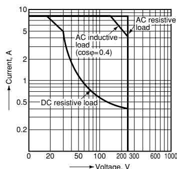
1. Max. switching power
