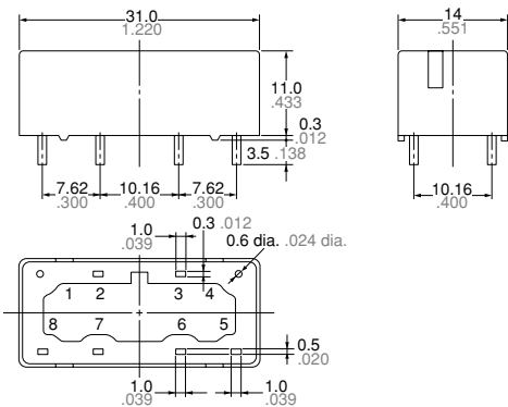
External dimensions
