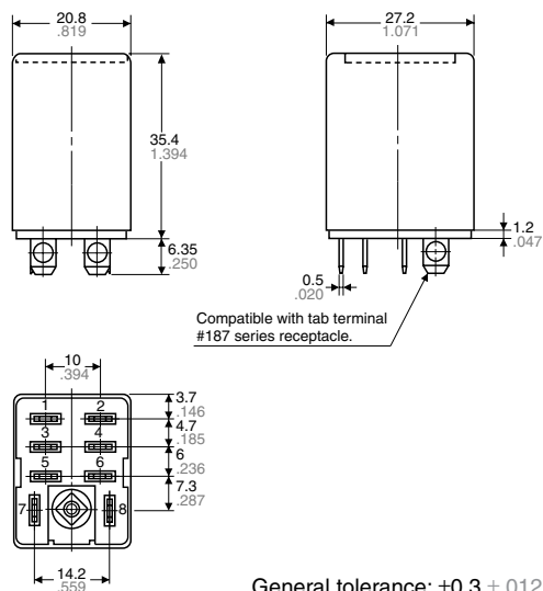
External dimensions
