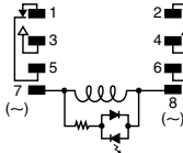
LED AC type
