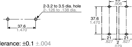
Chassis (Panel) cutout
