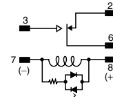
LED DC type
