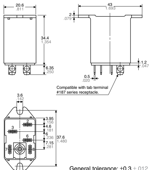
External dimensions
