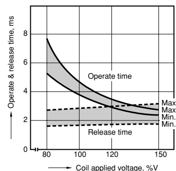
3.-(2) Operate & release time (1 Form C type)
