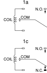
Schematic (Bottom view)
