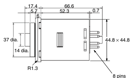
Dimensions with Back Connecting Socket P3G-08/P3GA-11
