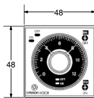
Dimensions with Back Connecting Socket P3G-08/P3GA-11
