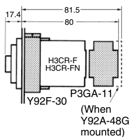
Dimensions with Back Connecting Socket P3G-08/P3GA-11
