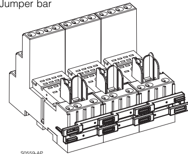
Jumper bar
