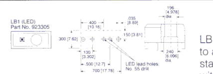
923305 LB1 (LED)
