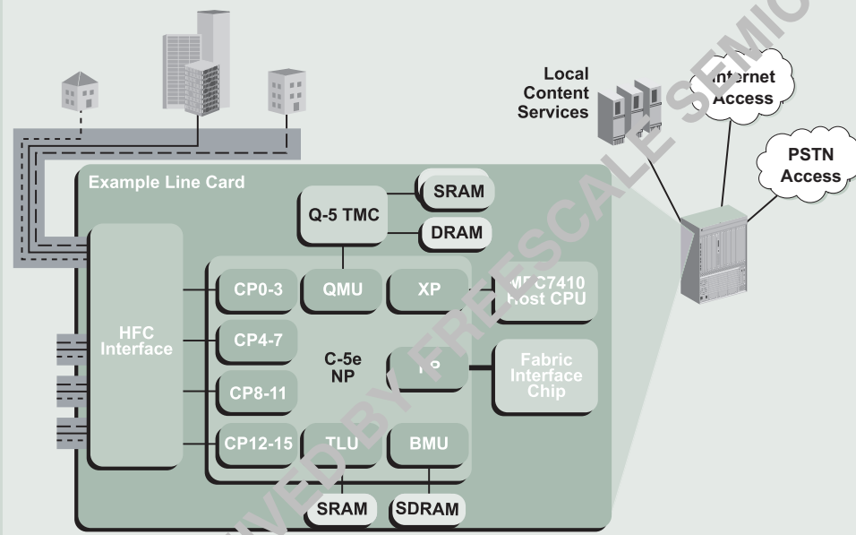
CMTS LINE CARD SOLUTION PROVIDING MULTI-PROTOCOL TRAFFIC MANAGEMENT
