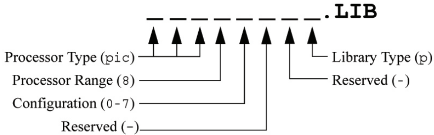
Figure 3.2: Peripheral Library Nomenclature
