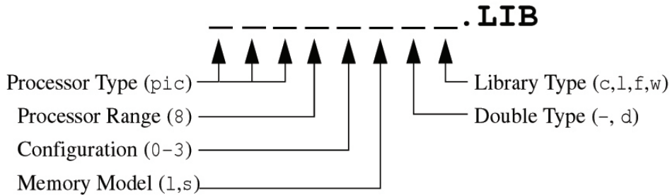
Figure 3.1: Library naming convention
