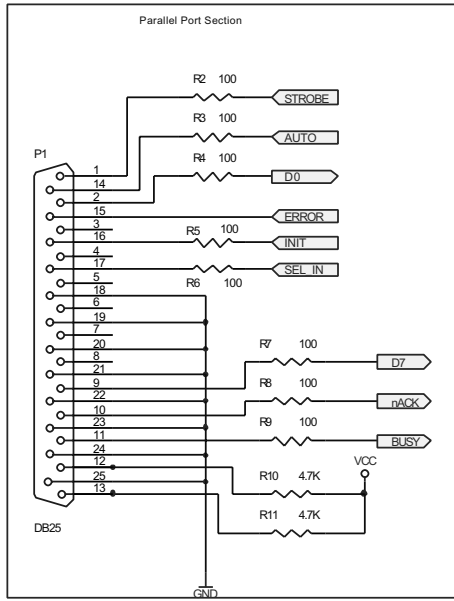
Figure 4-11. Schematic Diagram of Atmel CPLD ISP Cable, Continued
