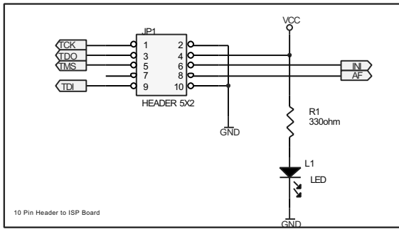
Figure 4-10. Schematic Diagram of Atmel CPLD ISP Cable
