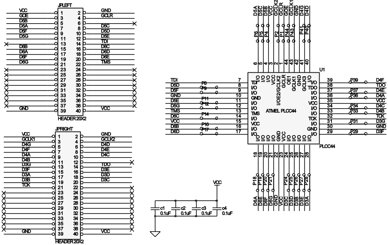
Figure 4-2. Schematic Diagram of 44-pin PLCC Socket Adapter Board
