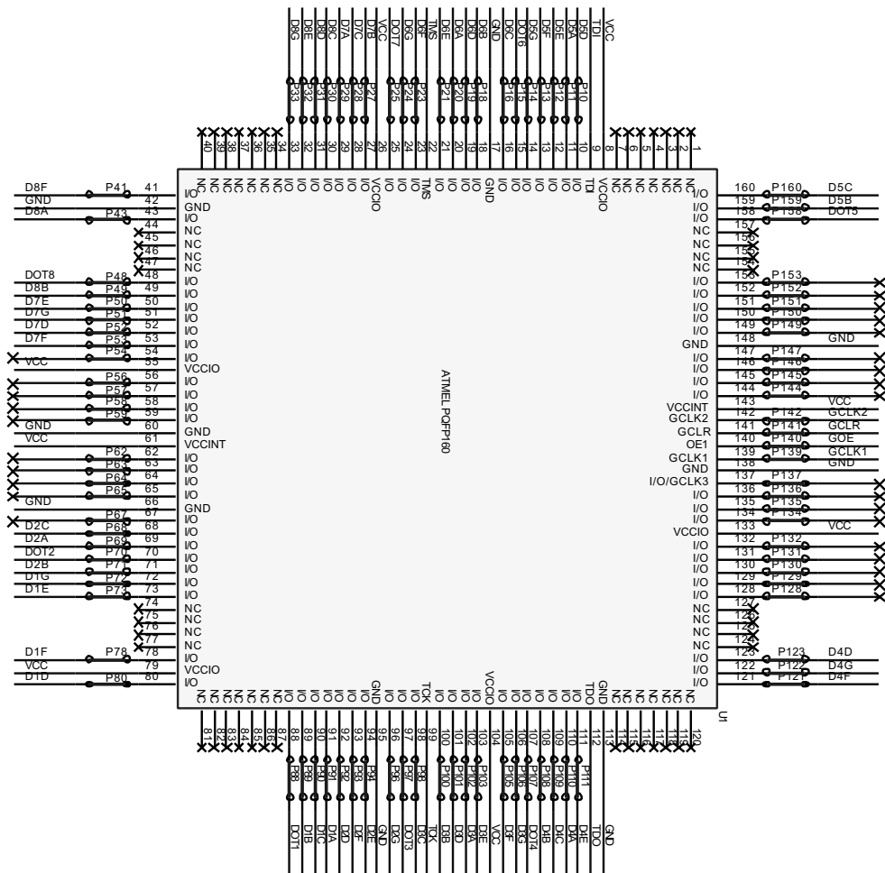
Figure 4-9. Schematic Diagram of 160-pin PQFP Socket Adapter Board
