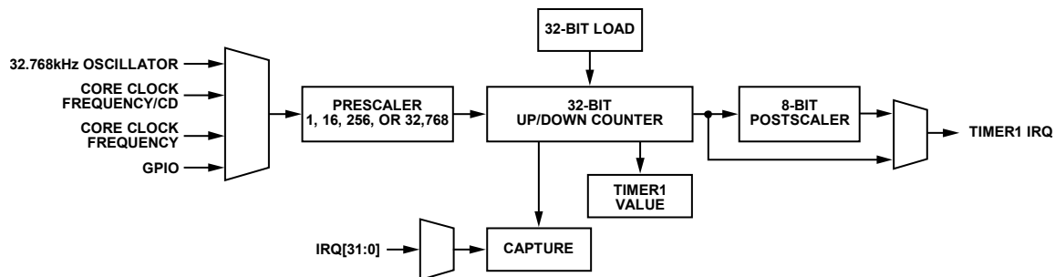
Figure 22. Timer0 Block Diagram
