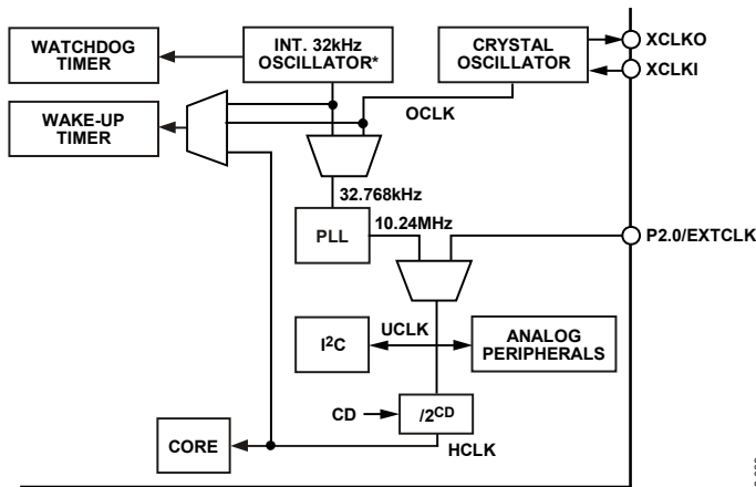
Figure 12. Clocking System
