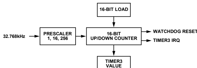
Figure 24. Timer2 Block Diagram
