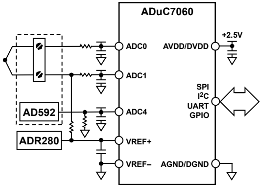
Figure 18. Example of a Thermocouple Interface Circuit
