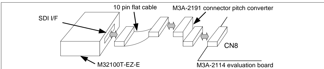
Figure 5.1-3 Connecting M3A-2114 Evaluation Board and M32100T-EZ-E
