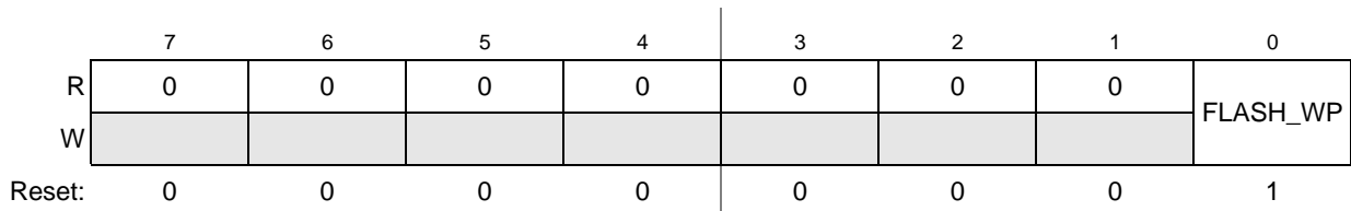
Figure 23. CPLD_FLASHCFG Register
