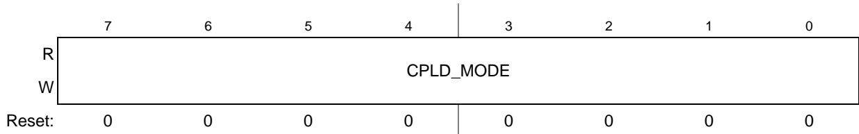
Figure 22. CPLD_MODE Register
