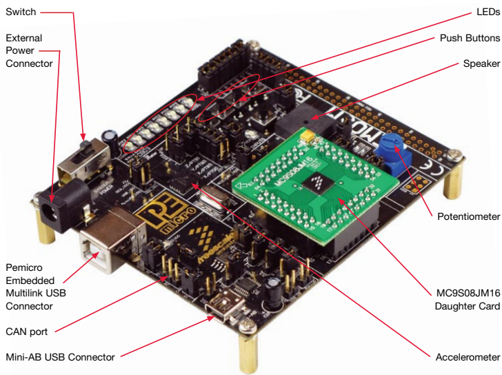
Figure 1. DEMOJM baseboard with MC9S08JM16 daughter card
