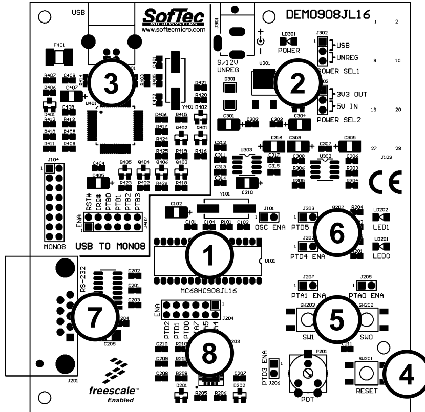
The DEMO908JL16 Demonstration Board
