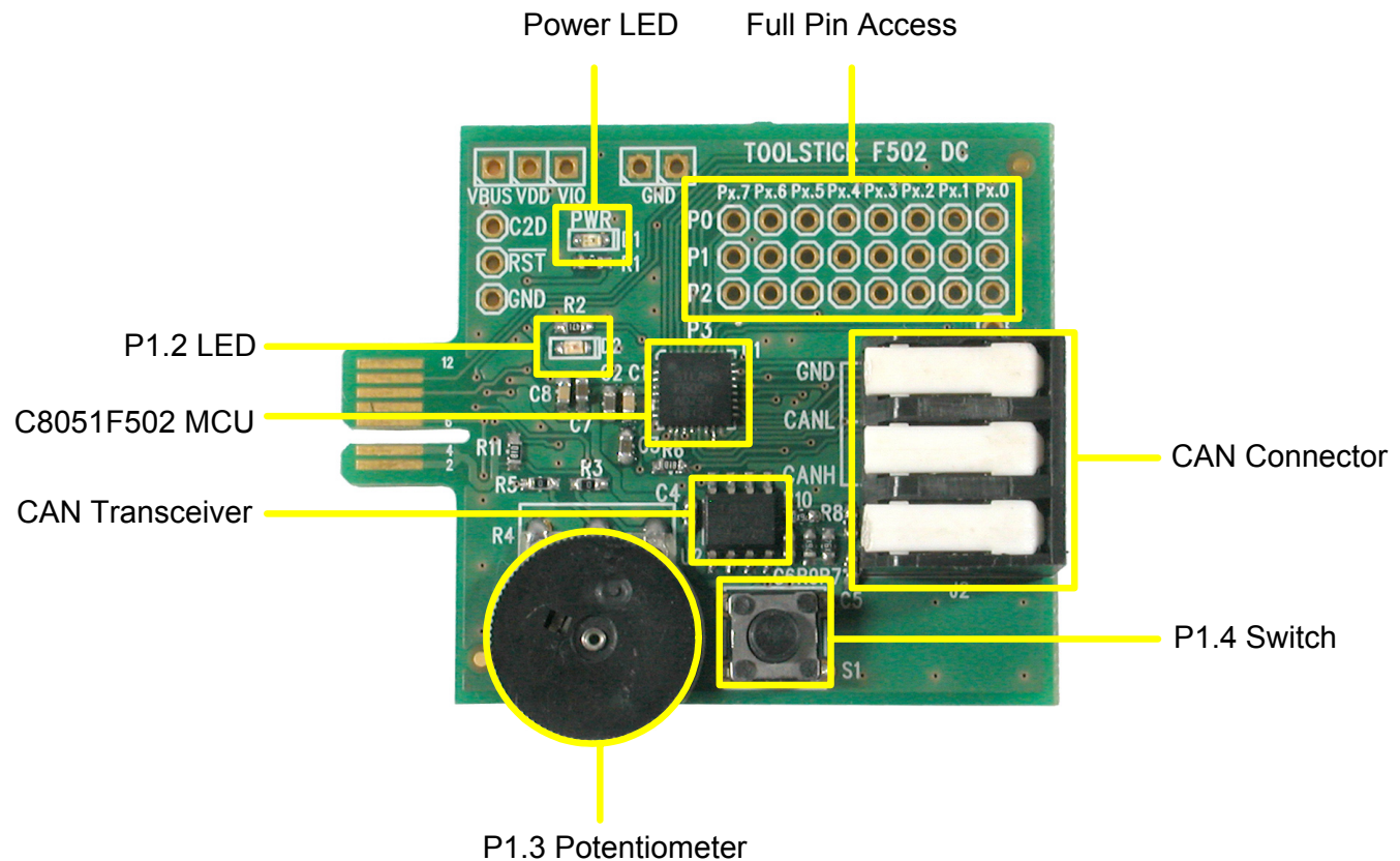
Figure 3. ToolStick C8051F502 Daughter Card
