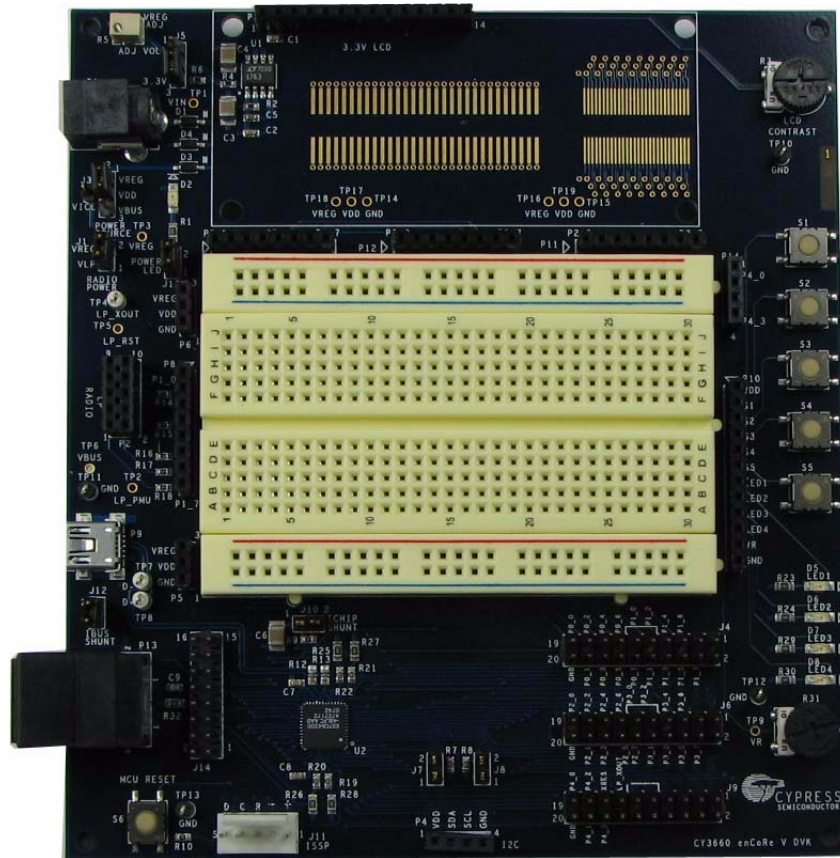
Figure 1-1. CY3660 Board
