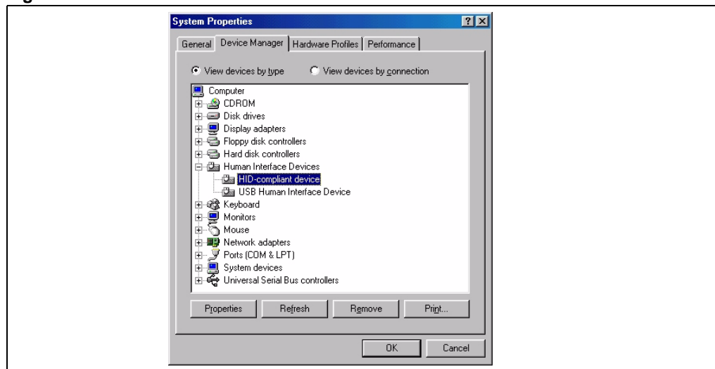
Figure 3. Enumeration result
