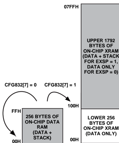
Figure 33. Extended Stack Pointer Operation
