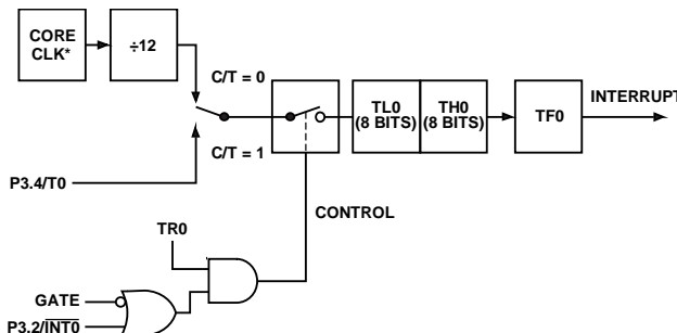
Figure 76. Timer/Counter 0, Mode 1
