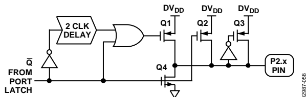
Figure 69. Internal Pull-Up Configuration
