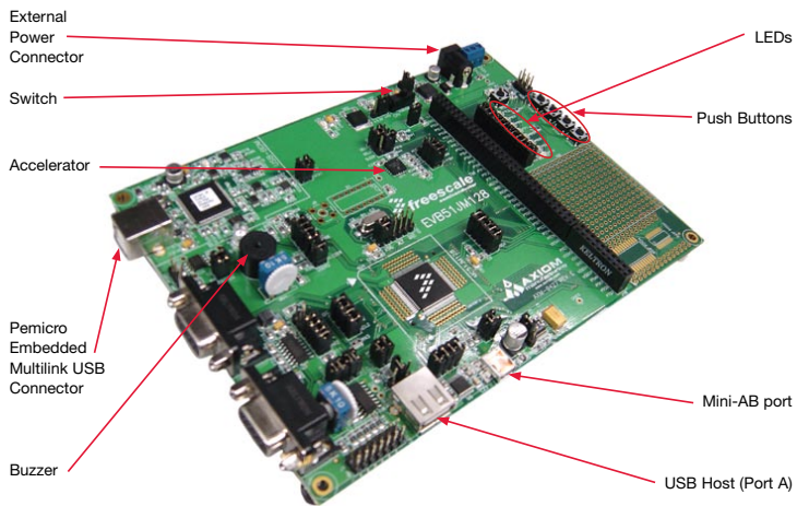
Figure 1. EVB51JM128 board
