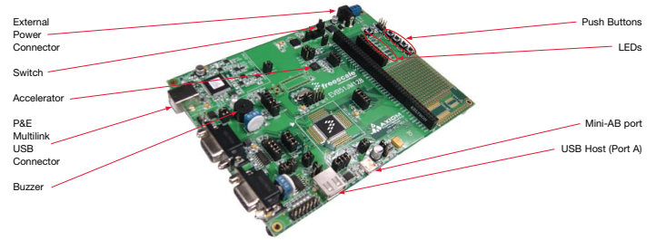
Figure 1. EVB51JM128 board
