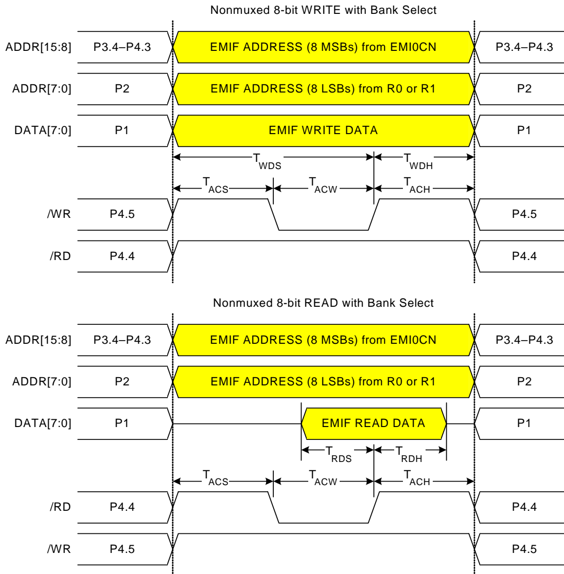
Figure 15.6. Non-multiplexed 8-bit MOVX with Bank Select Timing
