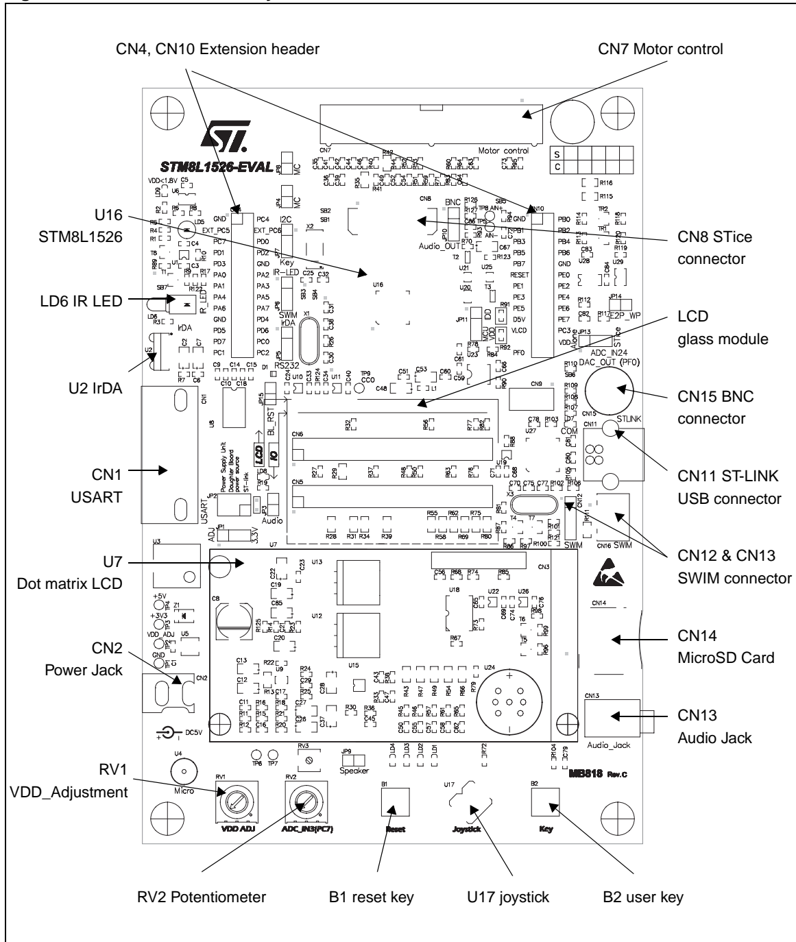
Figure 3. STM8L1526-EVAL layout
