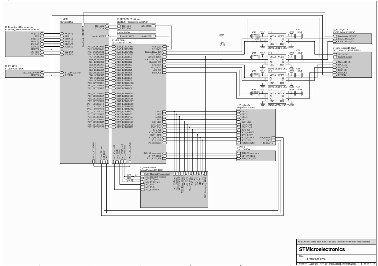
Figure 19. STM8L1526-EVAL
