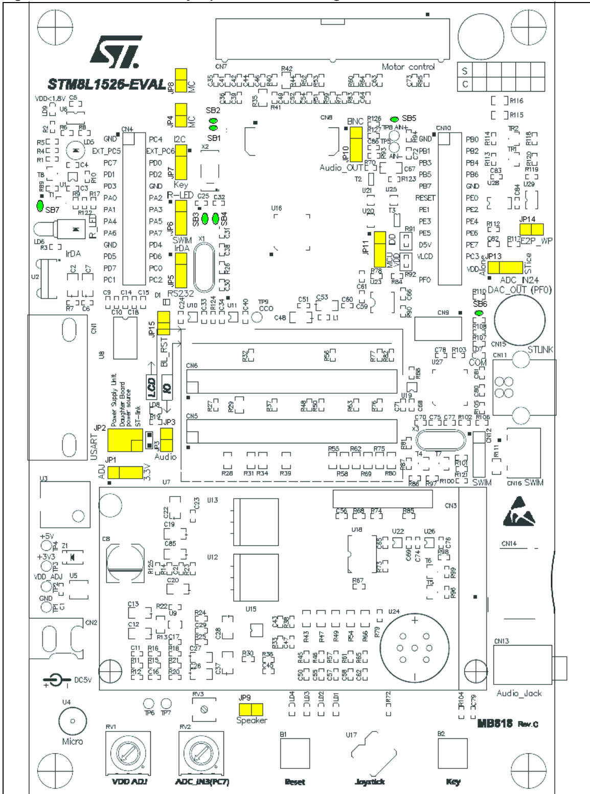
Figure 4. STM8L1526-EVAL jumpers and solder bridges
