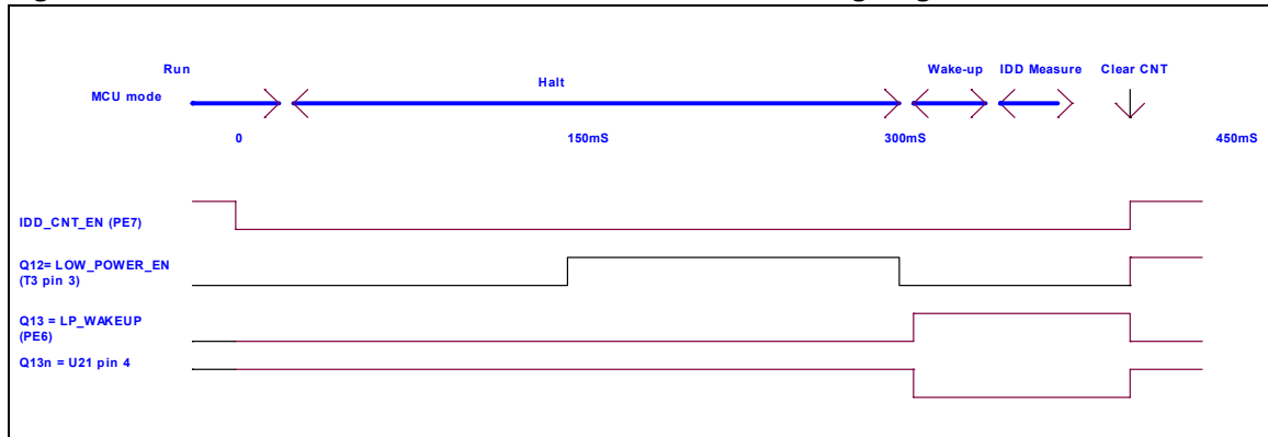
Figure 9. STM8L1526-EVAL IDD Halt mode measurement timing diagram
