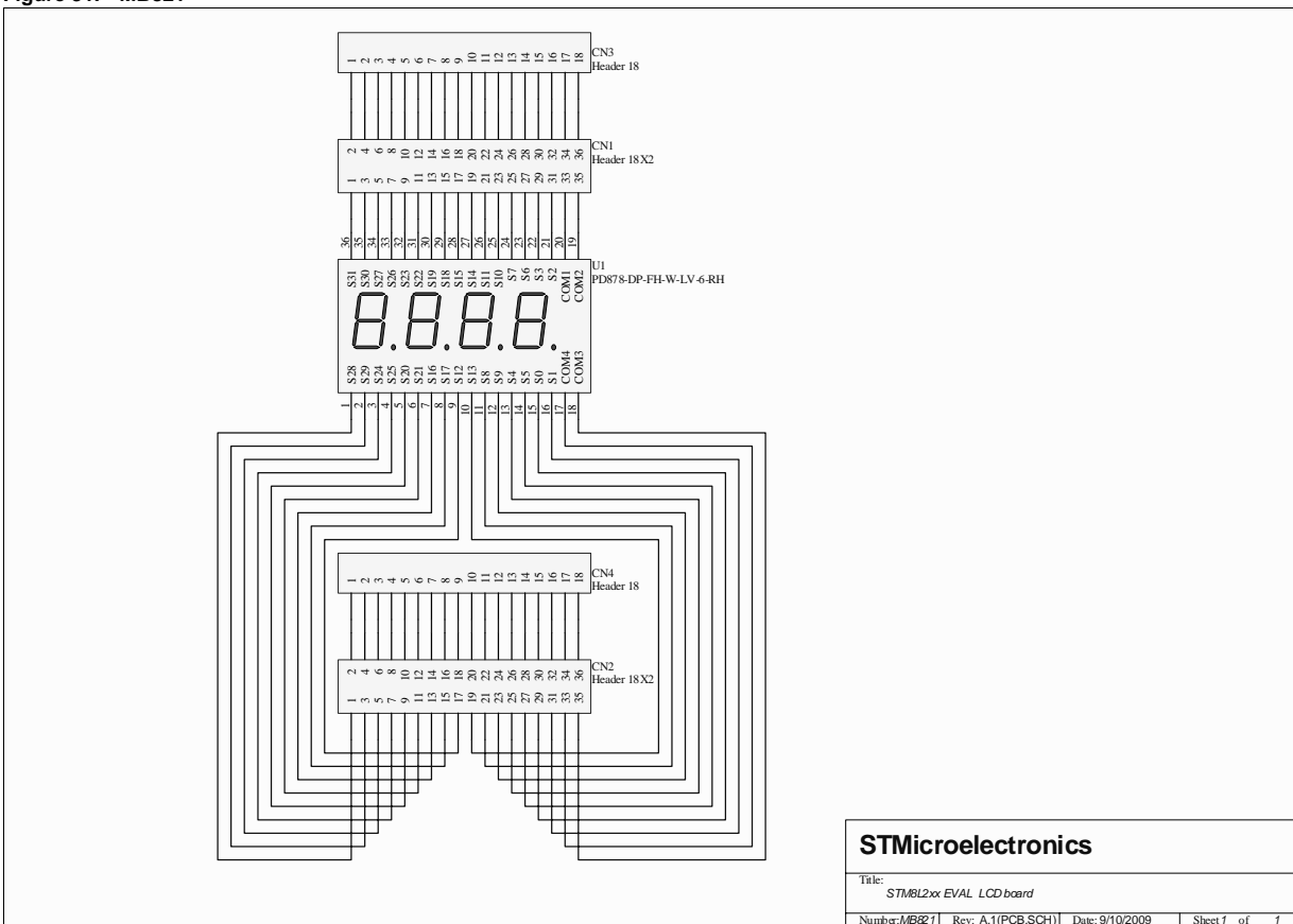
Figure 31. MB821
