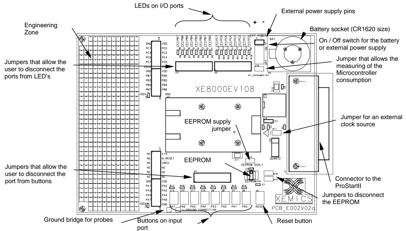
Figure 2 : Board elements
