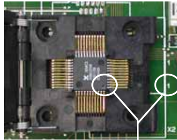
pin 1 markers
