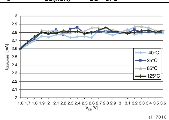
Figure 12. I_{DD(RUN)} vs. V_{DD} , f_{CPU} = 16\text{ MHz}
