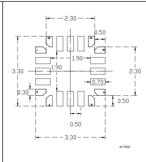
Figure 44. UFQFPN20 recommended footprint (1)(2)
