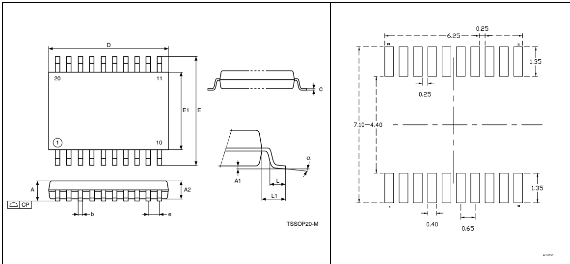
Figure 46. TSSOP20 recommended footprint (1)(2)
