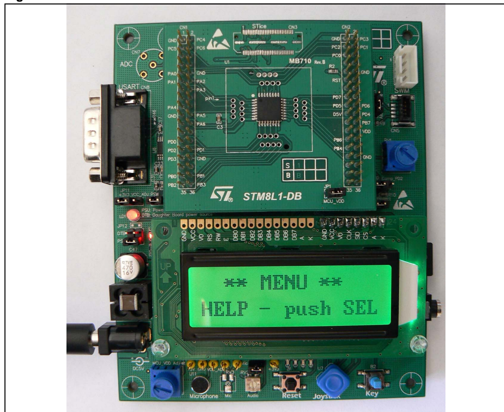
Figure 1. STM8L101-EVAL board
