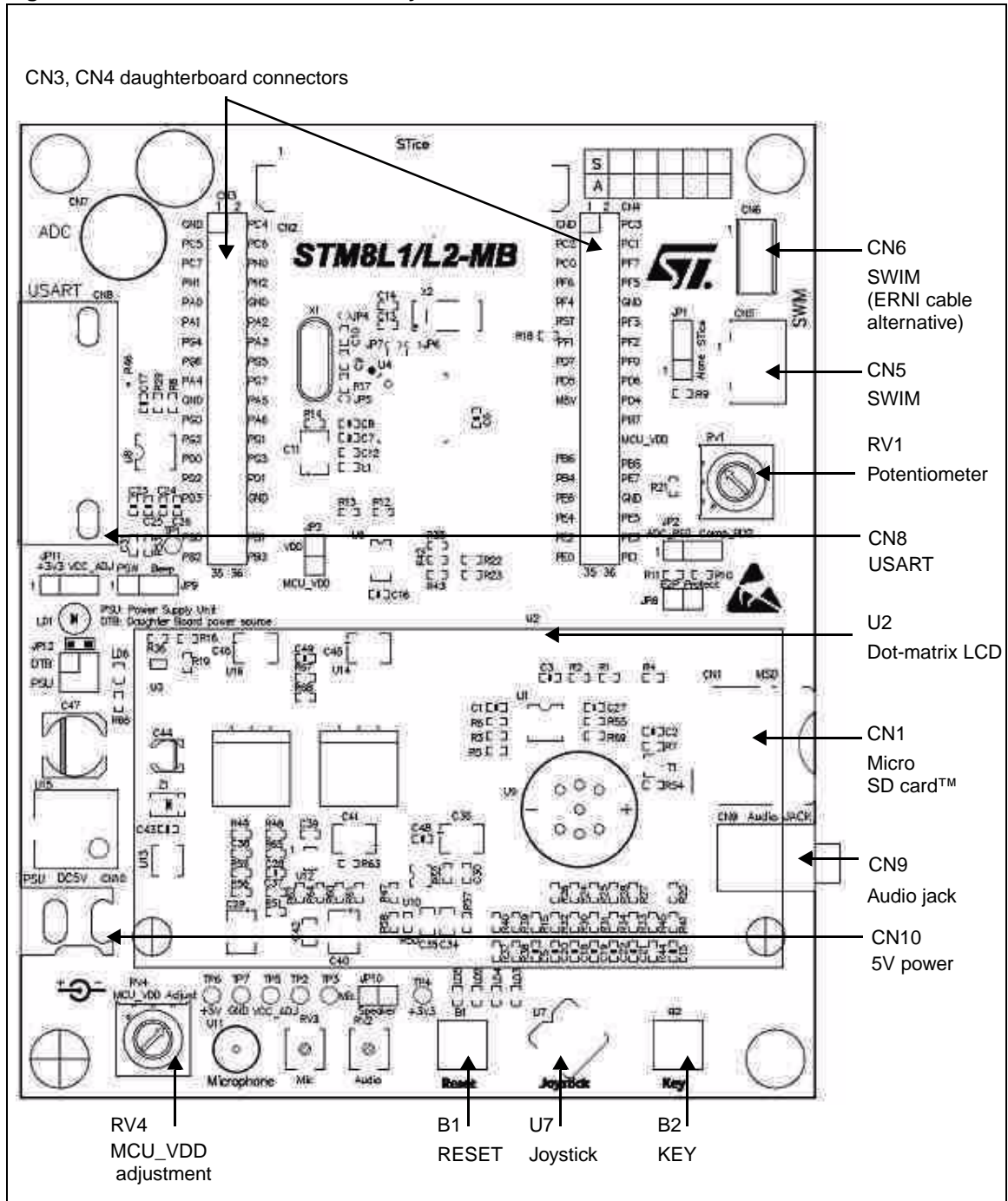
Figure 3. STM8L1/L2 motherboard layout
