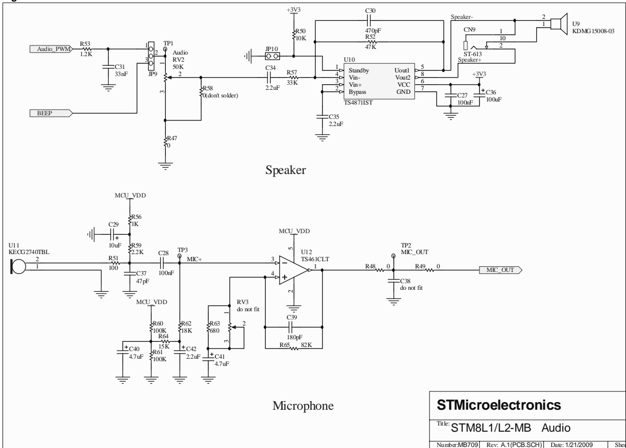
Figure 14. STM8L1/L2 motherboard audio
