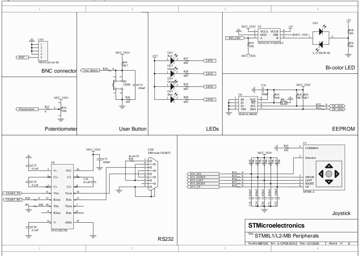
Figure 13. STM8L1 motherboard peripherals
