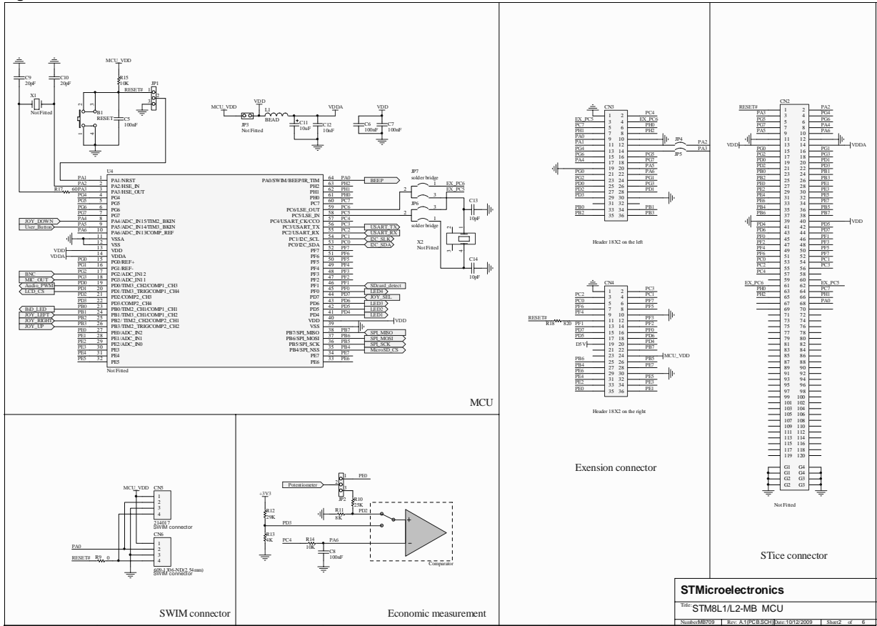
Figure 11. STM8L1 motherboard MCU
