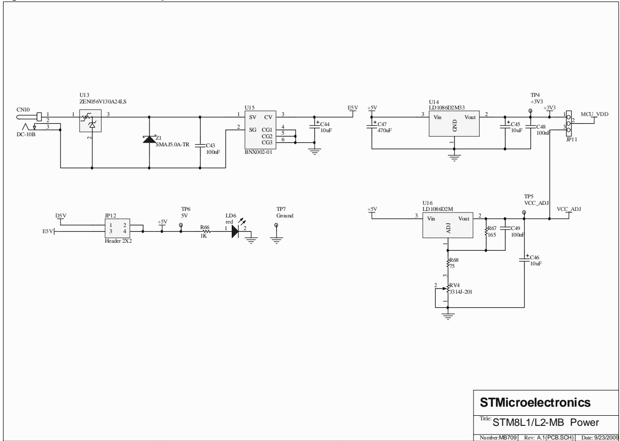
Figure 15. STM8L1 motherboard power
