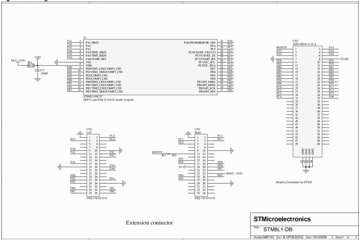
Figure 16. Daughterboard schematic
