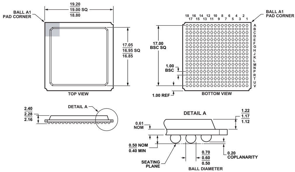
Figure 47. 324-Ball Plastic Ball Grid Array [PBGA]
