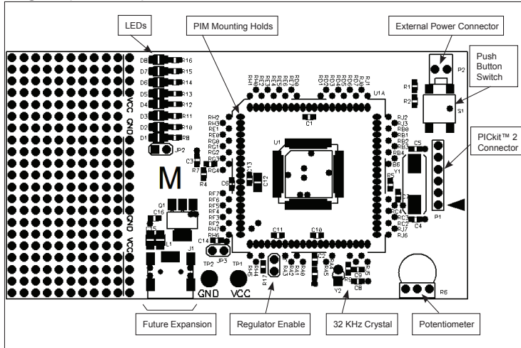
Figure 1: PICKit™ 2 64/80-Pin PIC18J Demonstration Board Diagram (DM4120-5)
