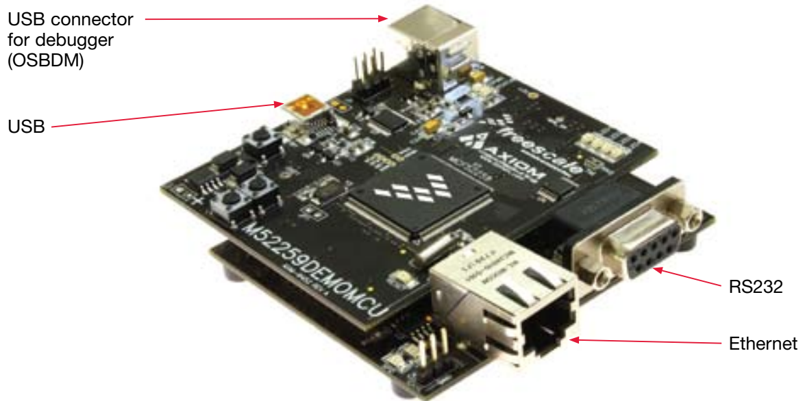
Figure 1. M52259DEMOKIT
