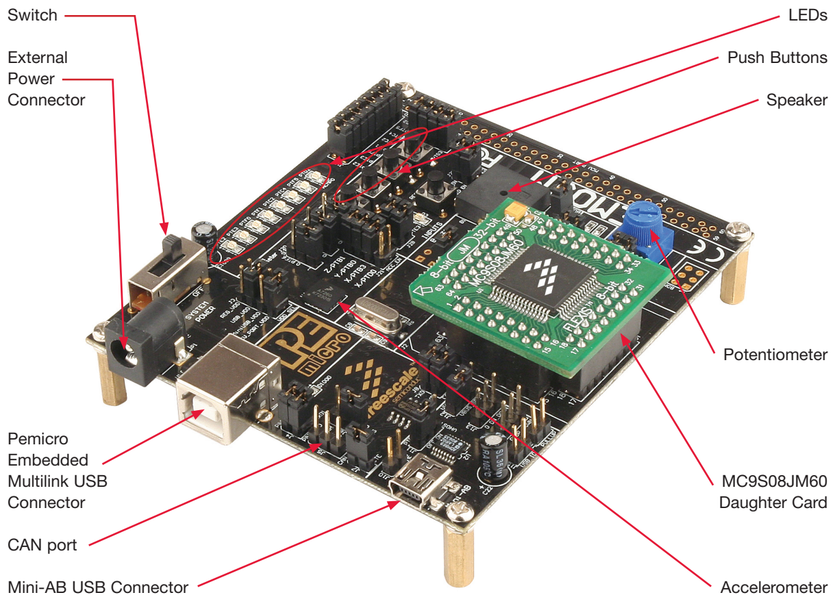
Figure 1. DEMOJM baseboard with MC9S08JM60 daughter card
