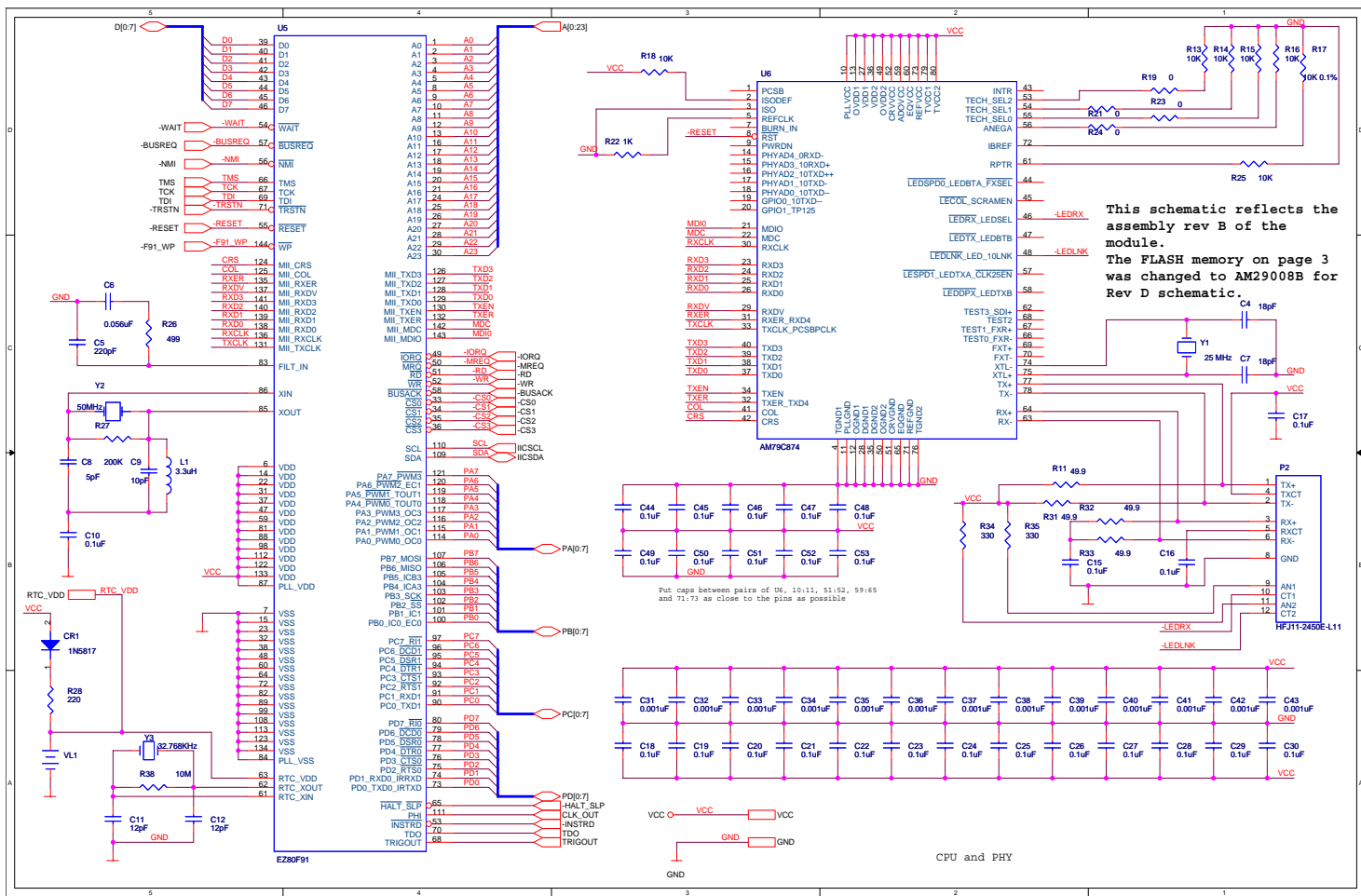
Figure 9. Zdots Schematic Diagram—CPU and PHY
