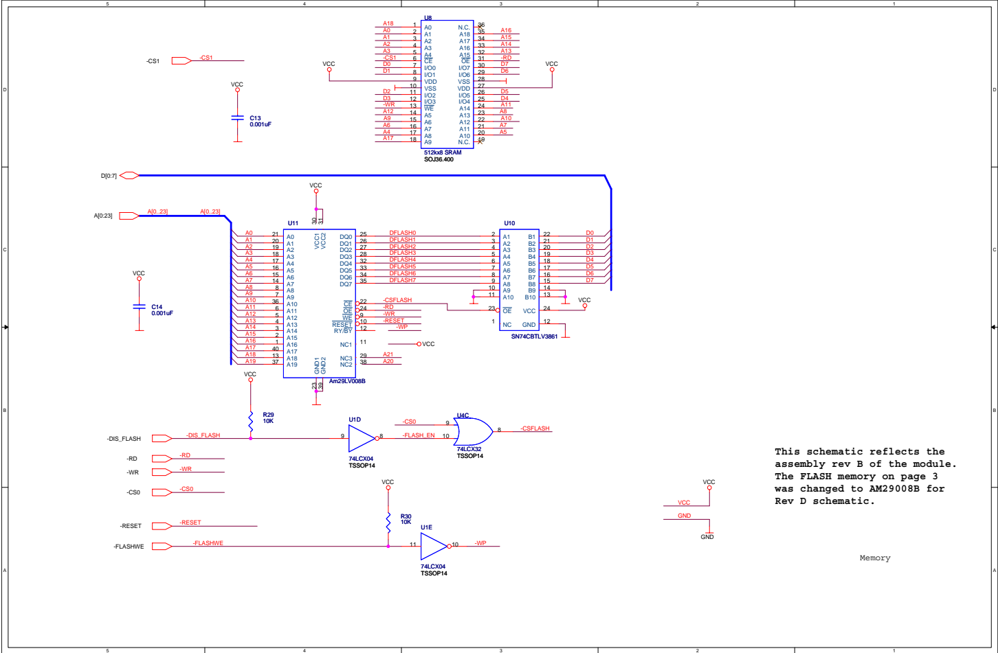
Figure 10. Zdots Schematic Diagram—Module Memory
