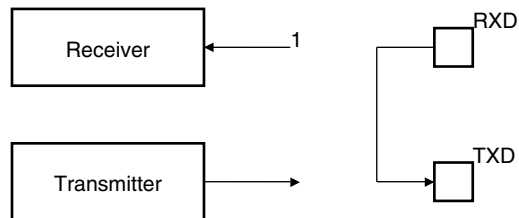
Figure 35-42. Remote Loopback Mode Configuration
