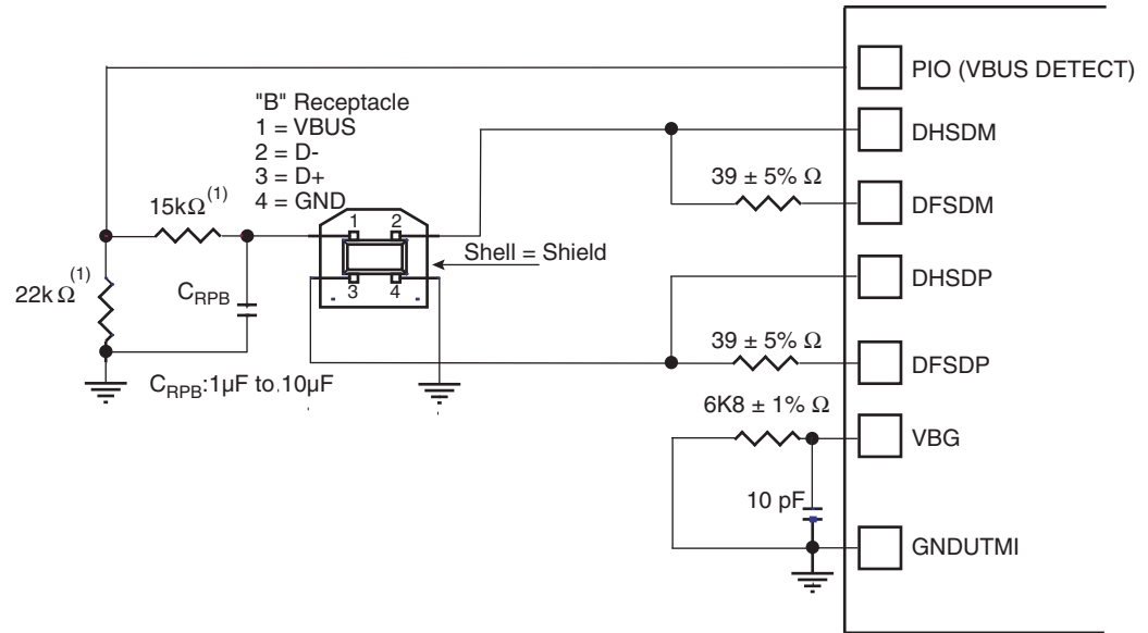
Figure 39-2. Board Schematic
