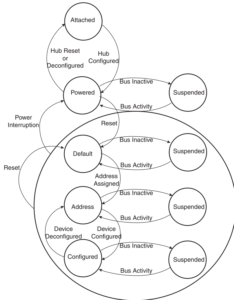
Figure 39-18. UDPHS Device State Diagram
