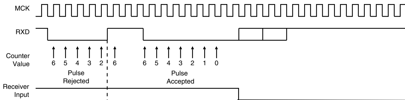
Figure 35-34. IrDA Demodulator Operations
