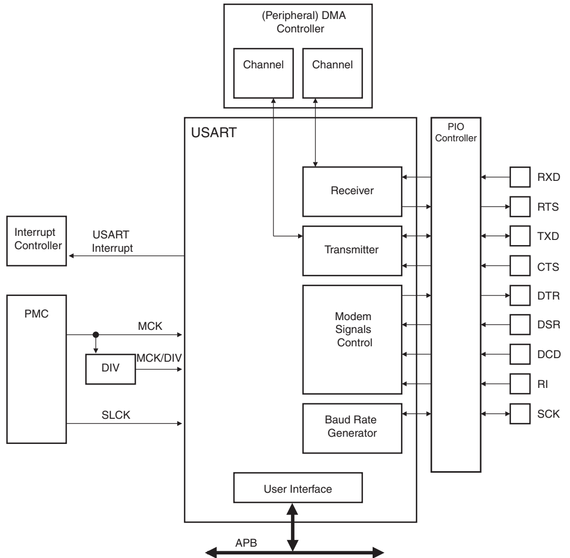
Figure 35-1. USART Block Diagram
