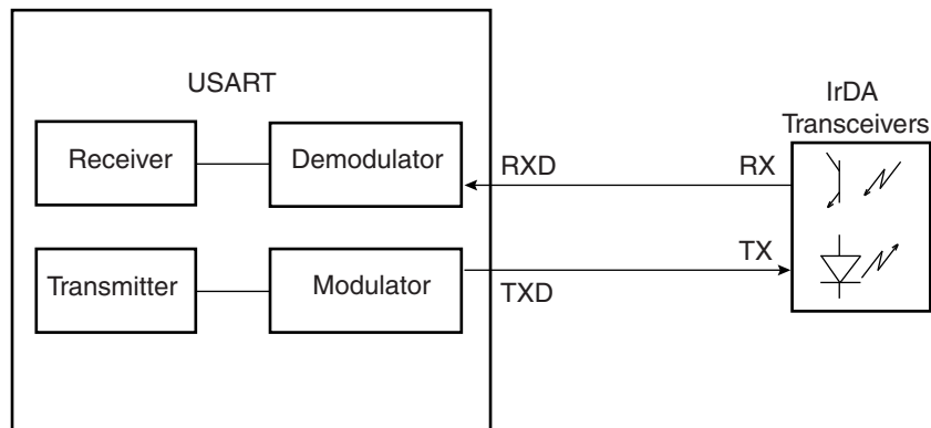
Figure 35-32. Connection to IrDA Transceivers
