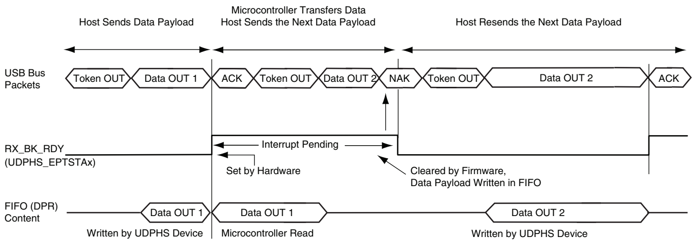
Figure 39-12. Data OUT Transfer for Endpoint with One Bank
