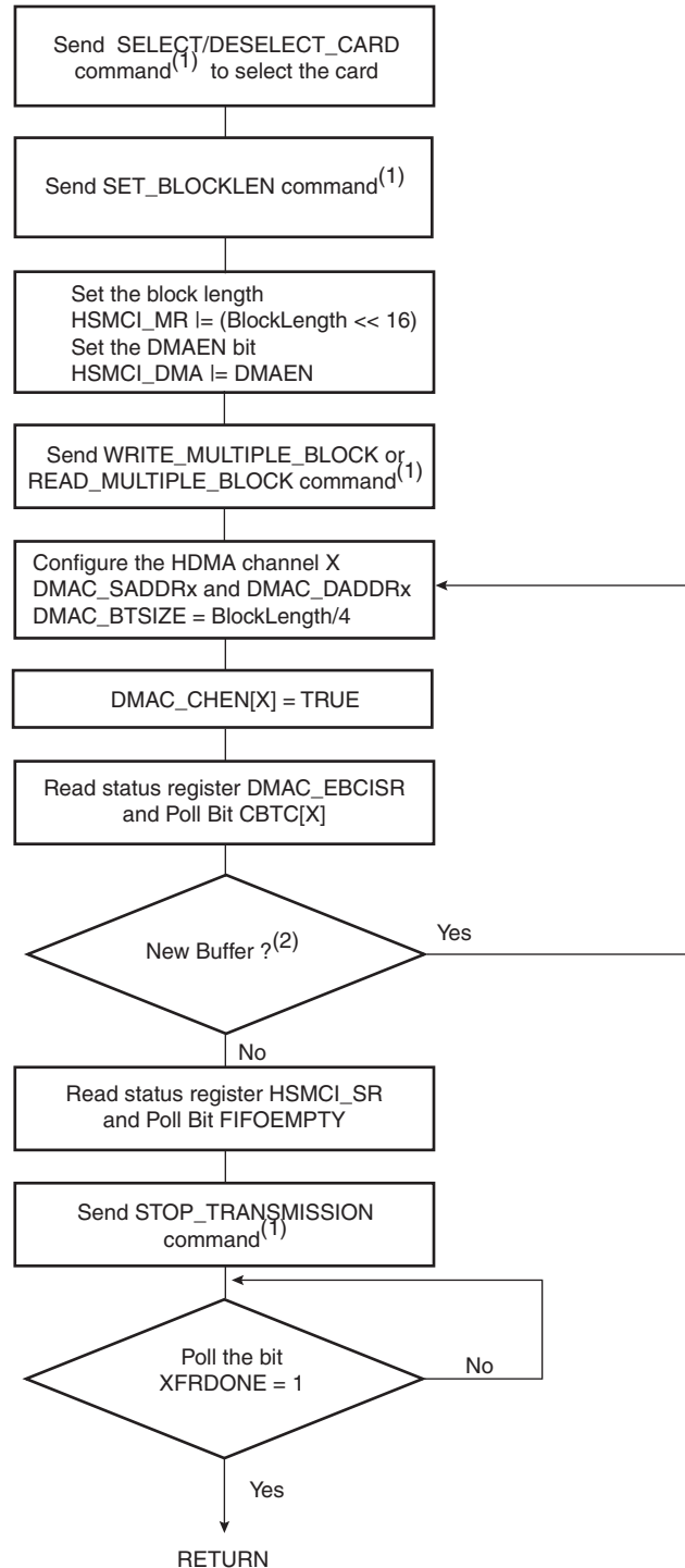
Figure 37-10. Read Multiple Block and Write Multiple Block
