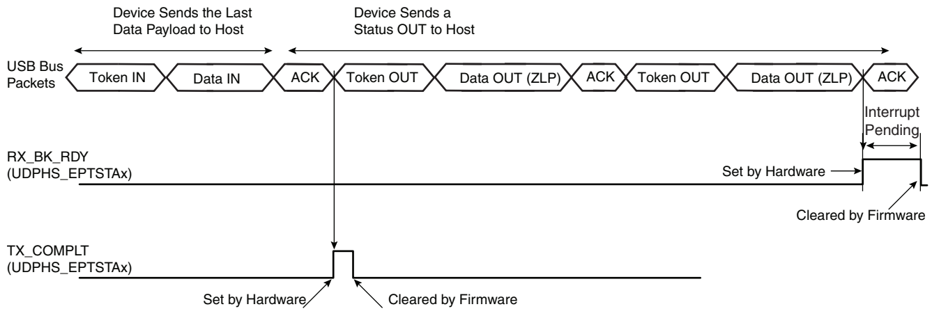
Figure 39-9. Data IN Followed By Status OUT Transfer at the End of a Control Transfer
