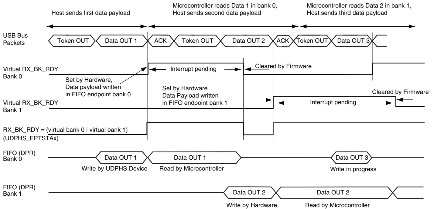
Figure 39-13. Data OUT Transfer for an Endpoint with Two Banks
