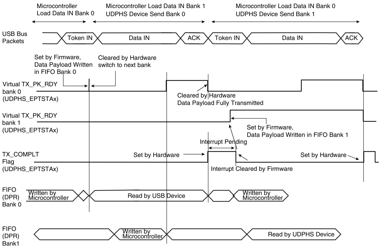
Figure 39-8. Data IN Transfer for Endpoint with Two Banks
