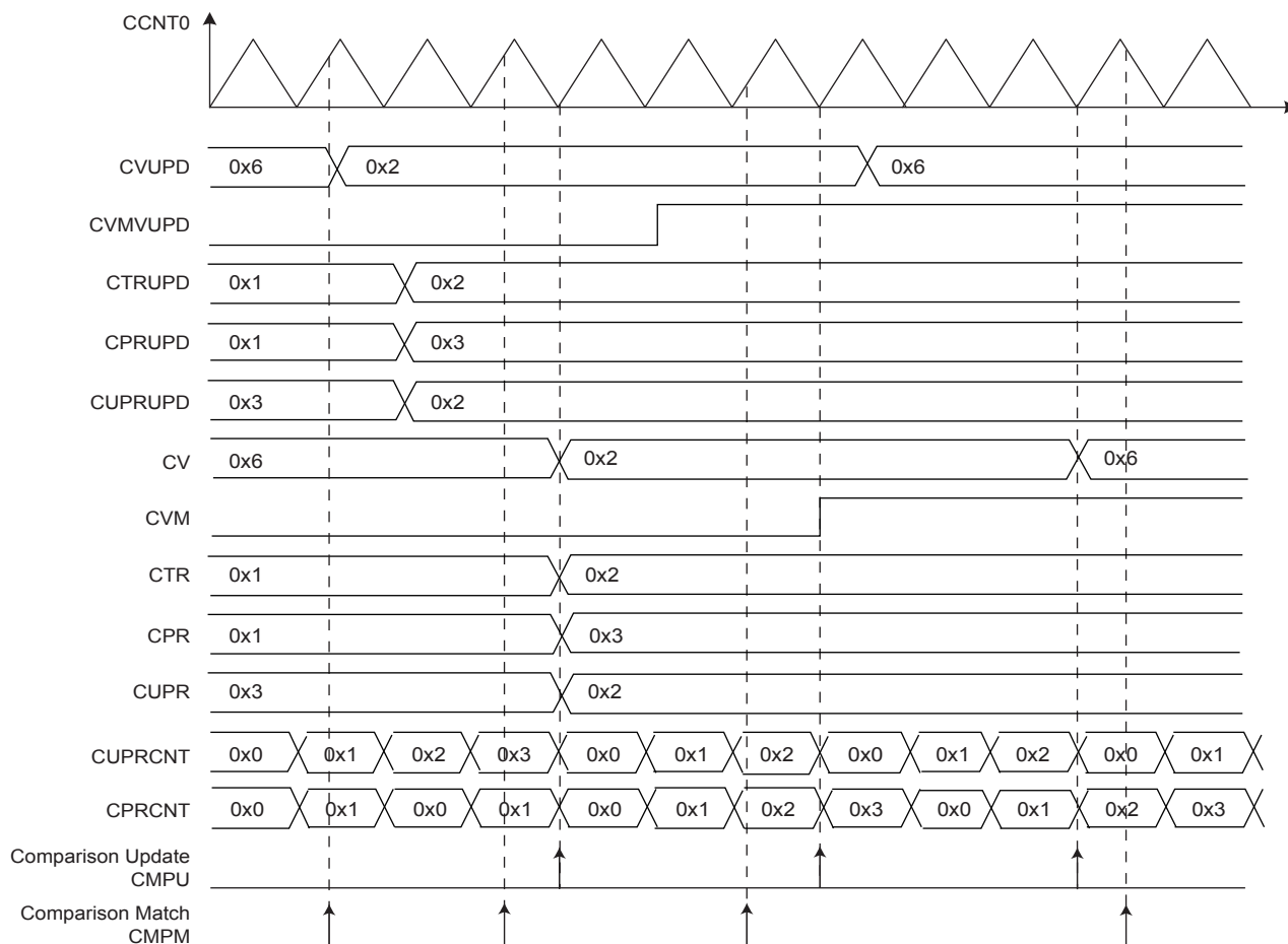
Figure 38-14. Comparison Waveform
