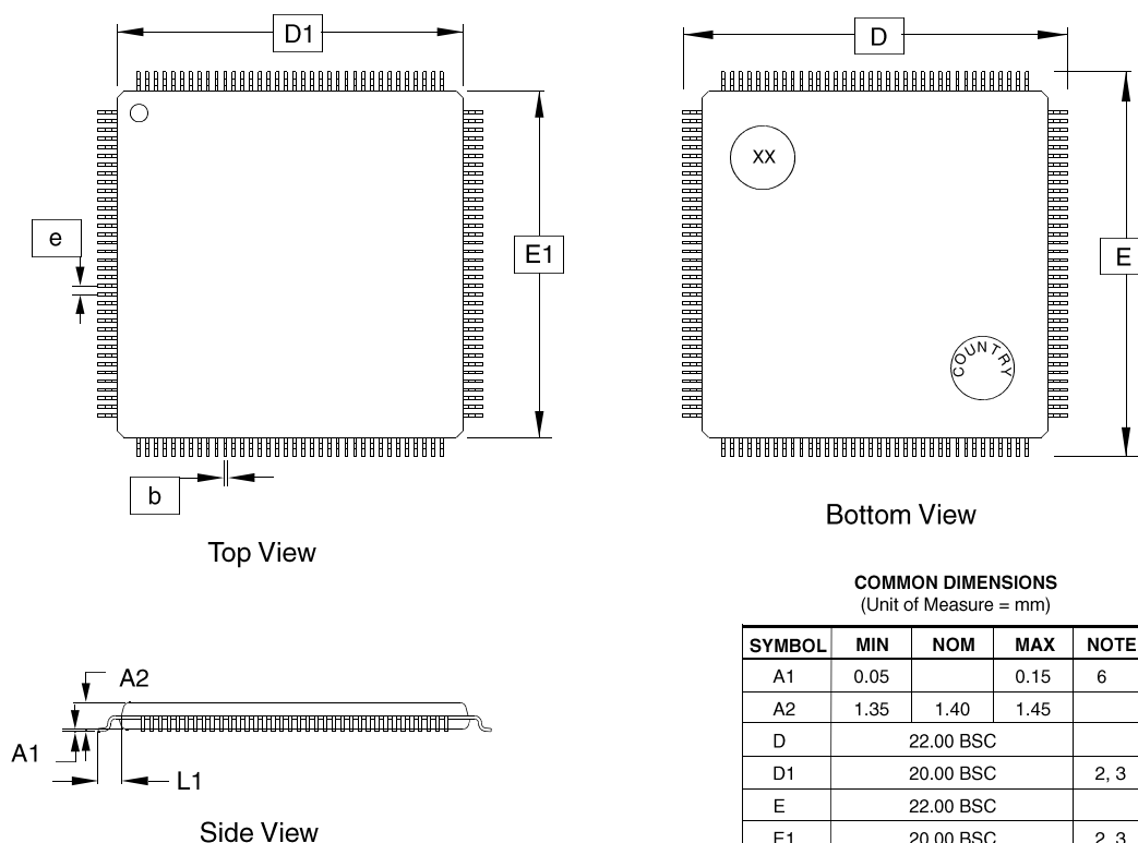
Figure 44-3. 144-lead LQFP Package Drawing
