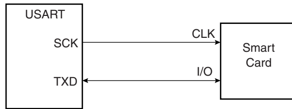
Figure 35-29. Connection of a Smart Card to the USART
