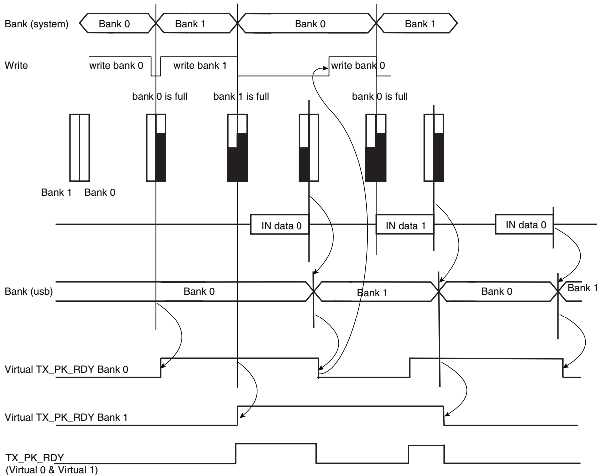
Figure 39-11. Autovalid with DMA
