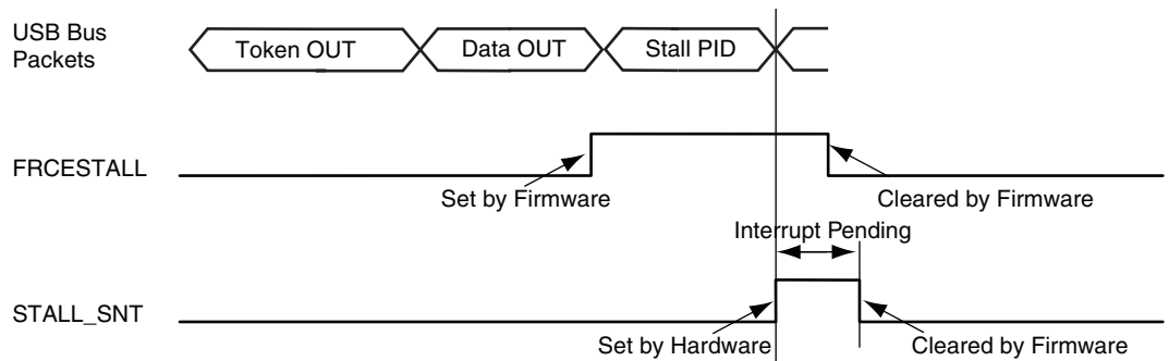
Figure 39-15. Stall Handshake Data OUT Transfer
