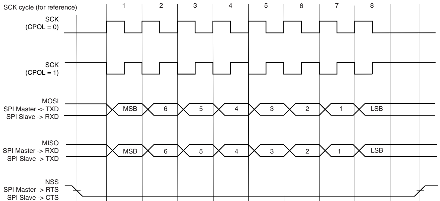
Figure 35-38. SPI Transfer Format (CPHA=0, 8 bits per transfer)
