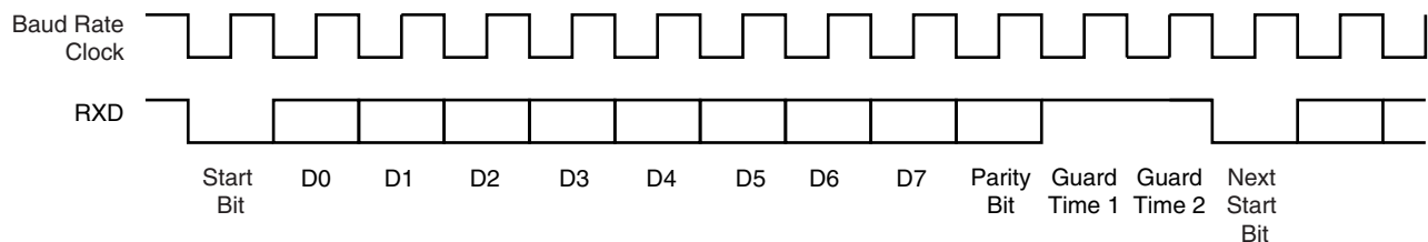
Figure 35-30. T = 0 Protocol without Parity Error
