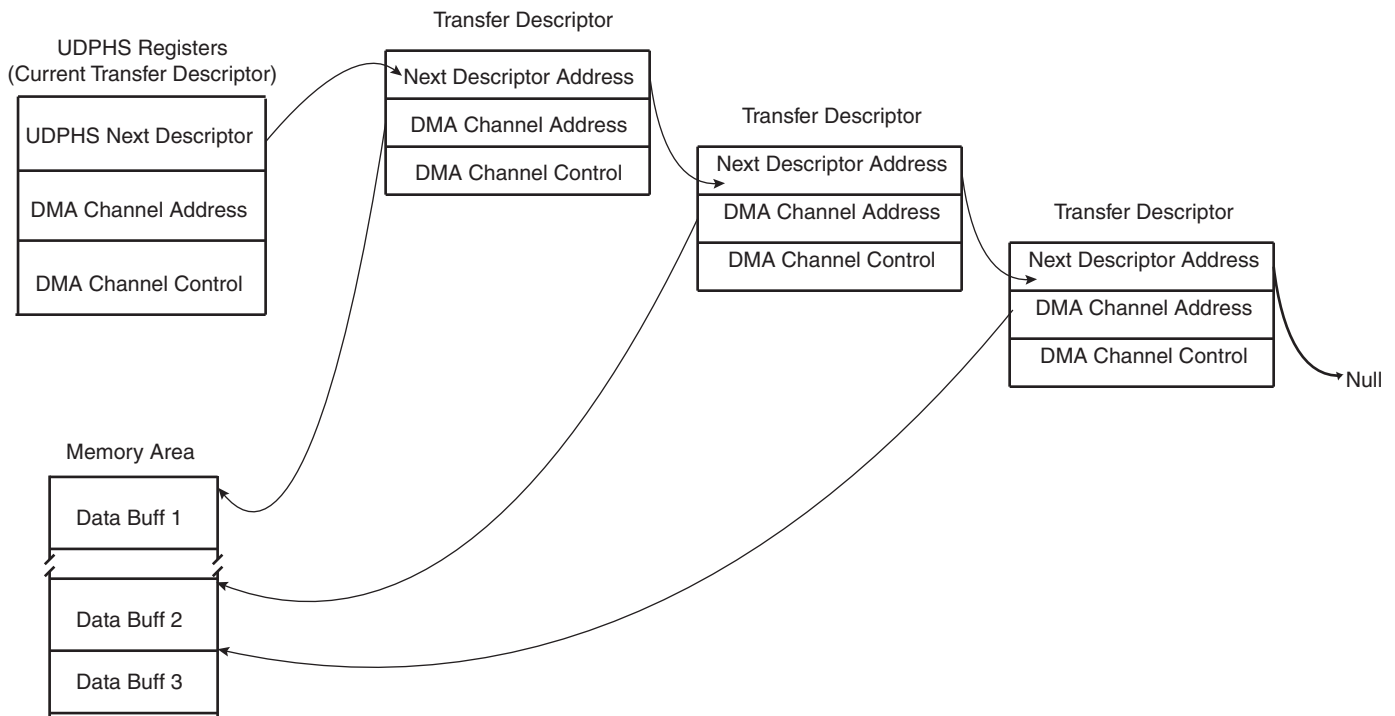
Figure 39-5. Example of DMA Chained List
