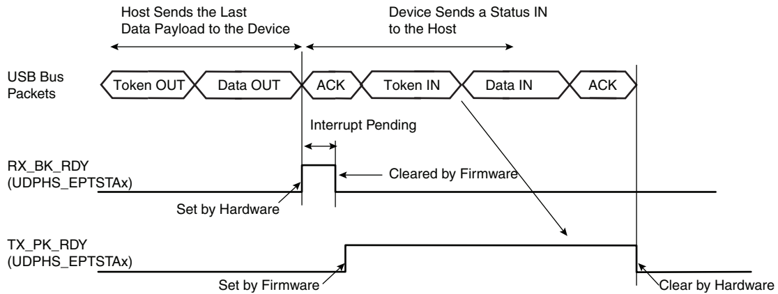
Figure 39-10. Data OUT Followed by Status IN Transfer
