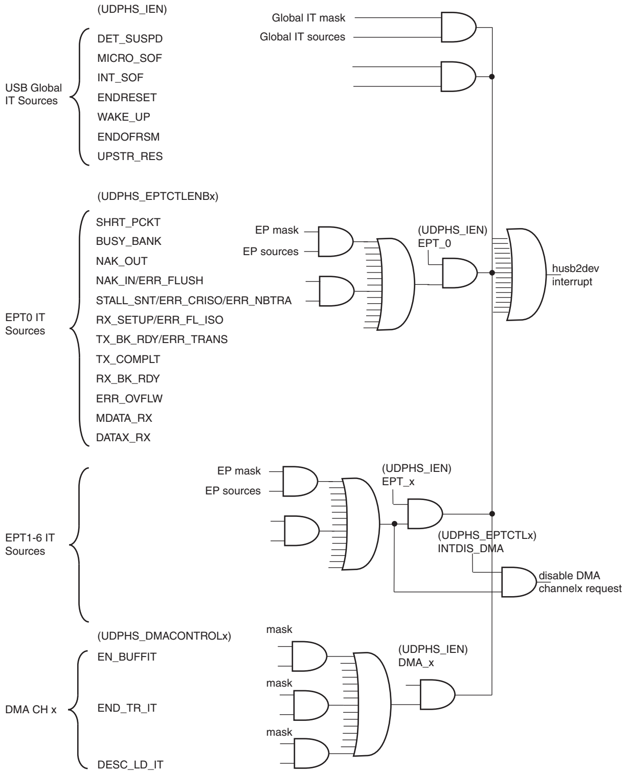
Figure 39-17. UDPHS Interrupt Control Interface
