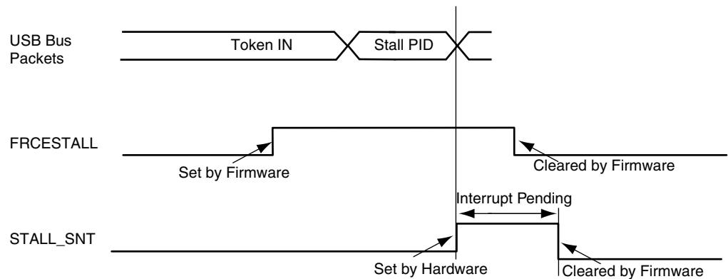
Figure 39-16. Stall Handshake Data IN Transfer
