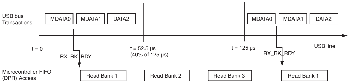
Figure 39-14. Bank Management, Example of Three Transactions per Microframe
