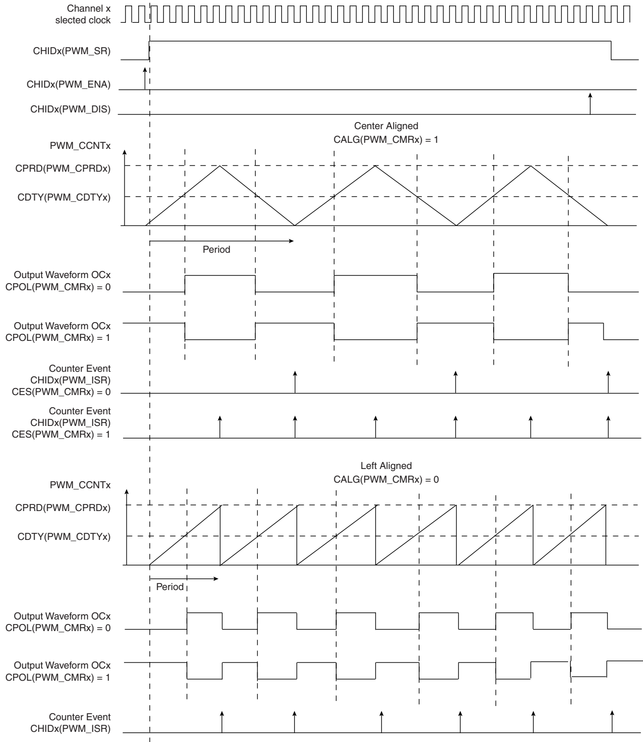
Figure 38-5. Waveform Properties
