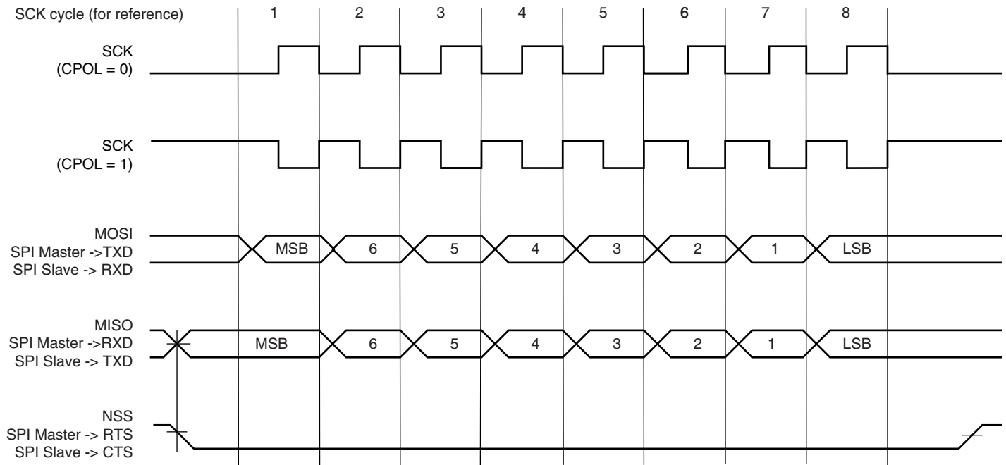
Figure 35-37. SPI Transfer Format (CPHA=1, 8 bits per transfer)
