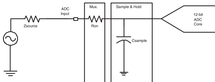
Figure 43-10. Simplified Acquisition Path
