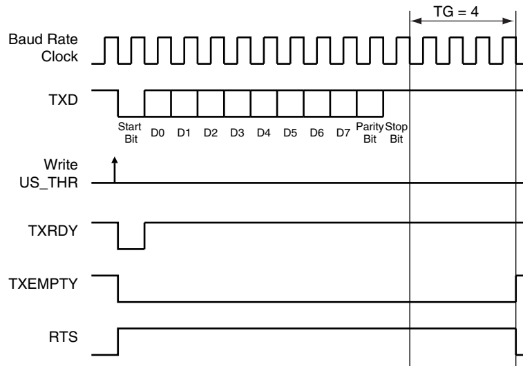
Figure 35-36. Example of RTS Drive with Timeguard
