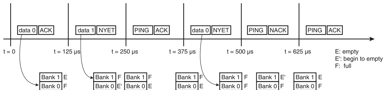
Figure 39-6. NYET Example with Two Endpoint Banks
