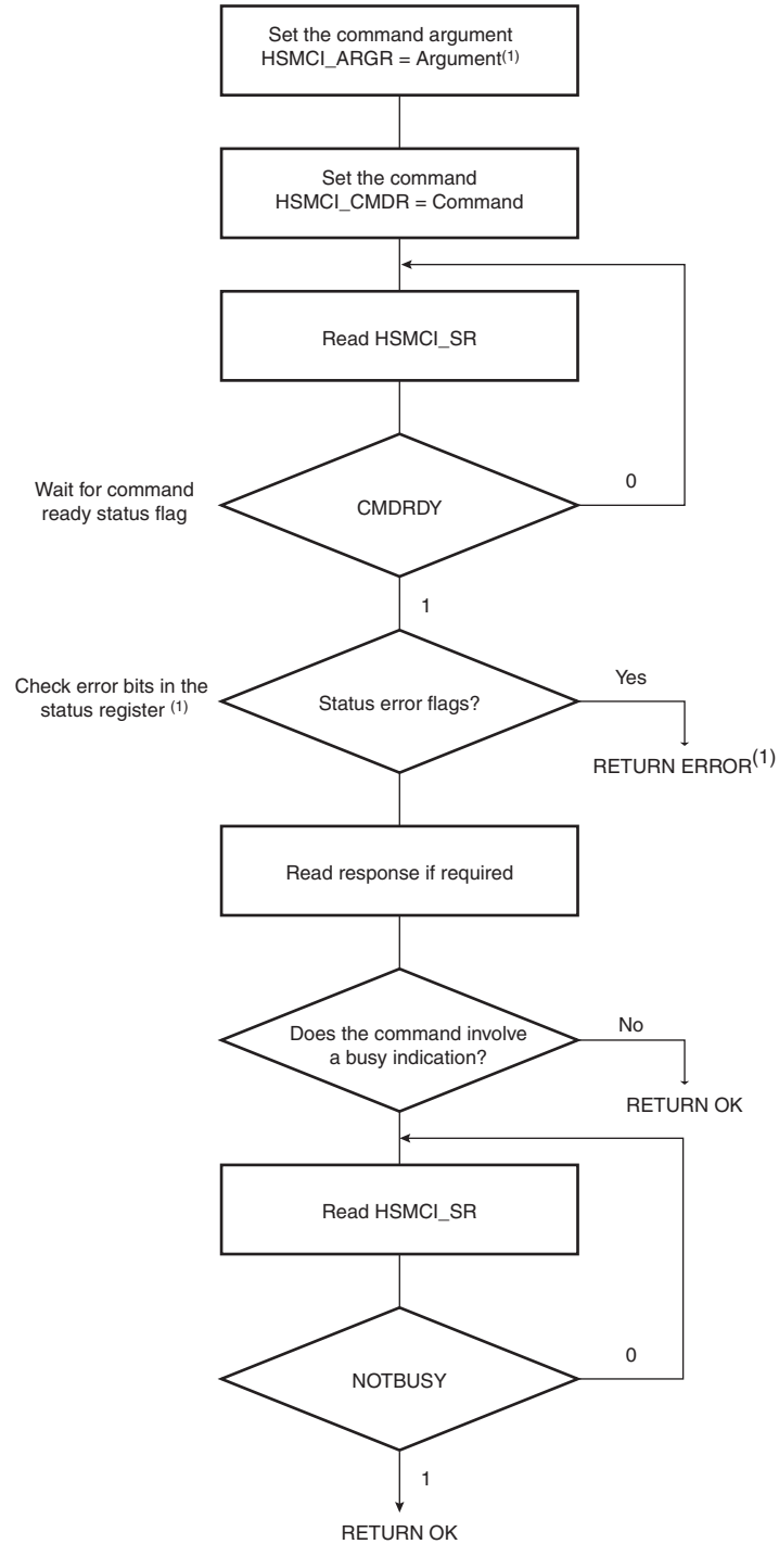
Figure 37-7. Command/Response Functional Flow Diagram
