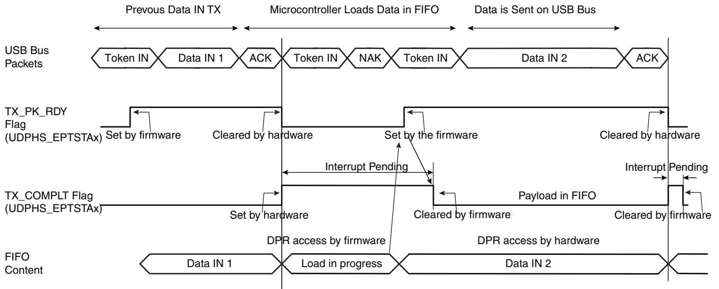
Figure 39-7. Data IN Transfer for Endpoint with One Bank
