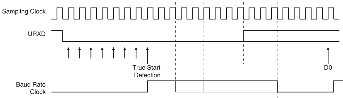
Figure 34-3. Start Bit Detection
