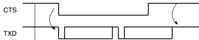
Figure 35-28. Transmitter Behavior when Operating with Hardware Handshaking
