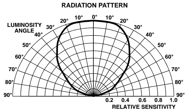
FIGURE 10. RADIATION PATTERN
