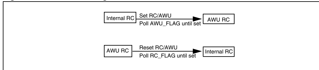
Figure 9. Clock switching
