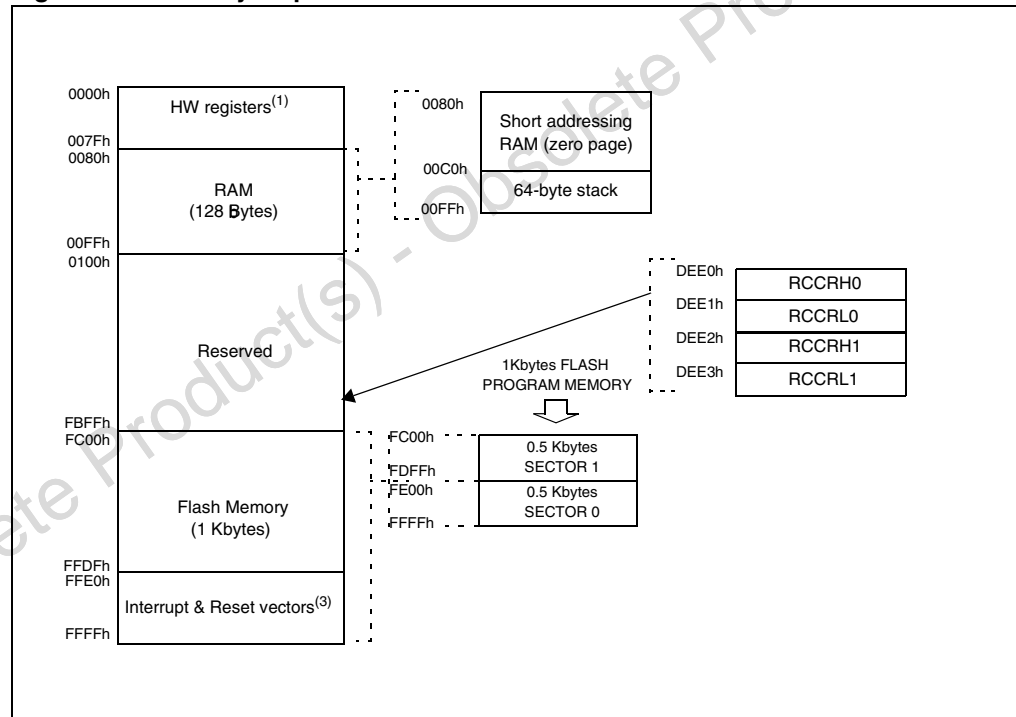
Figure 5. Memory map
