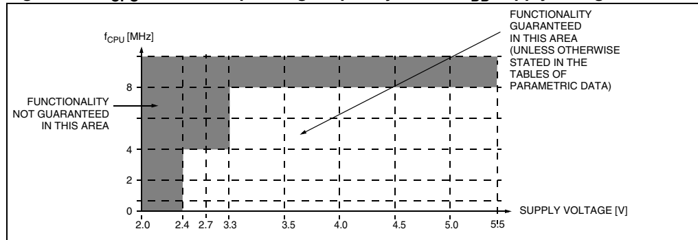
Figure 39. f_{\text{CPU}} maximum operating frequency versus V_{\text{DD}} supply voltage
