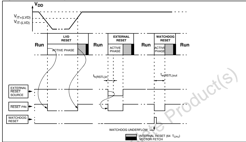
Figure 13. Reset sequences
