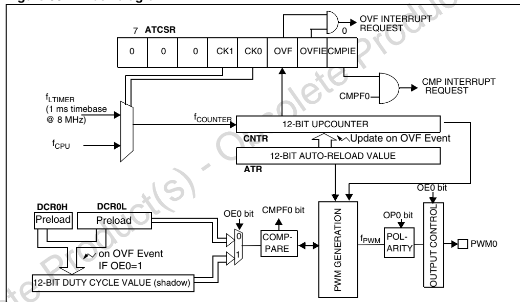
Figure 33. Block diagram
