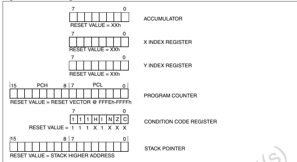
Figure 7. CPU registers
