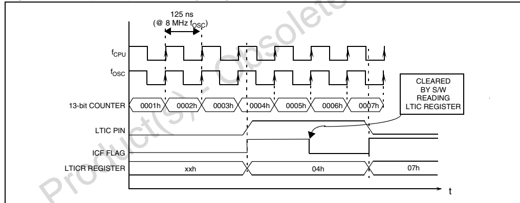
Figure 32. Input capture timing diagram
