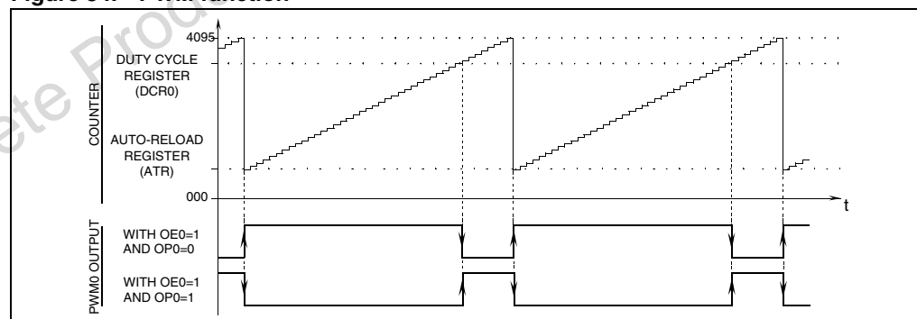
Figure 34. PWM function
