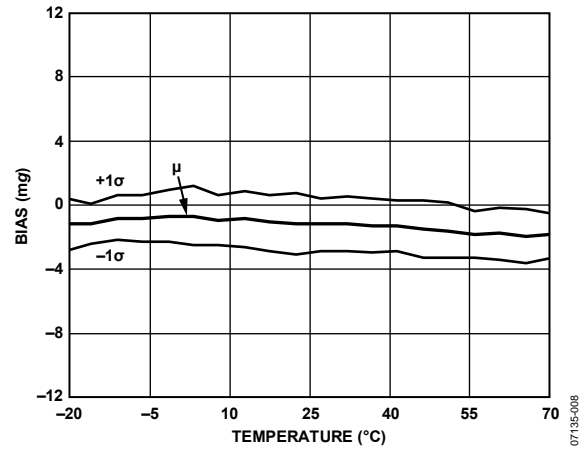
Figure 9. Accelerometer Bias vs. Temperature
