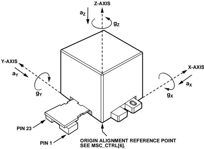
Figure 4. Pin Configuration
