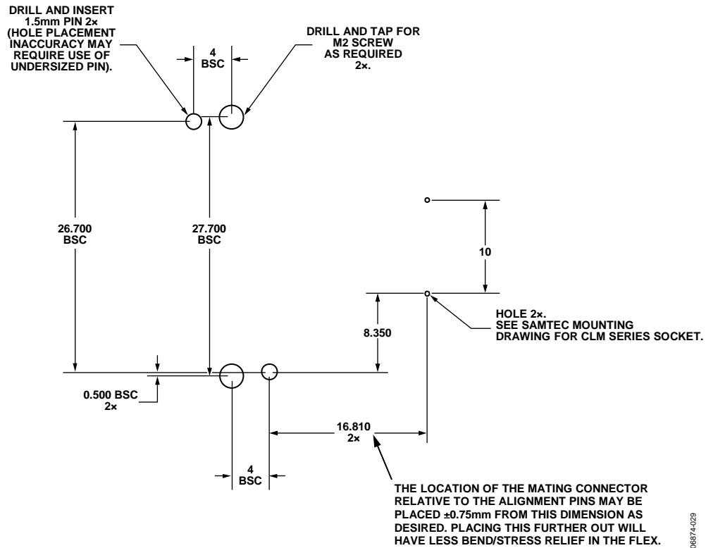
Figure 29. Hole Locations
