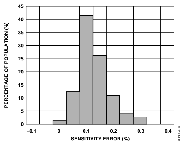
Figure 16. Gyroscope Sensitivity Error, +25°C
