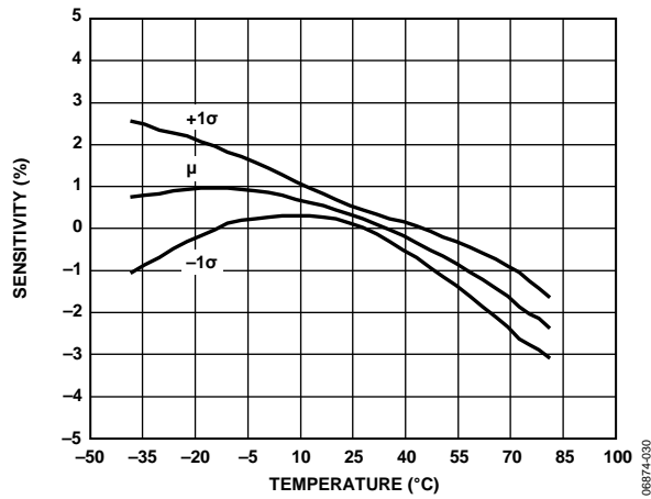
Figure 6. ADIS16350 Gyroscope Sensitivity vs. Temperature
