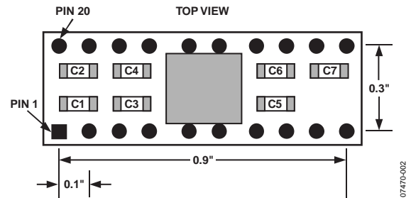
Figure 2. EVAL-ADXRS610 Parts Layout
