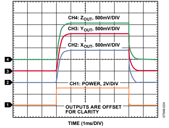
Figure 22. Typical Turn-On Time, V_S = 3\text{ V} , C_X = C_Y = C_Z = 0.0047\text{ }\mu\text{F}
