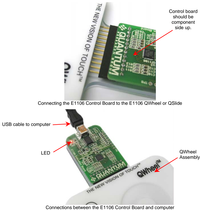
Figure 2: E1106 Connections
