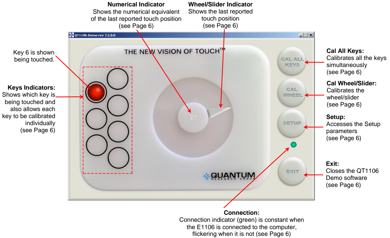
Figure 3: QT1106 Main Window
