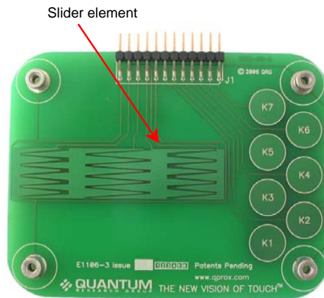
Figure 8: QSlide Assembly Details
