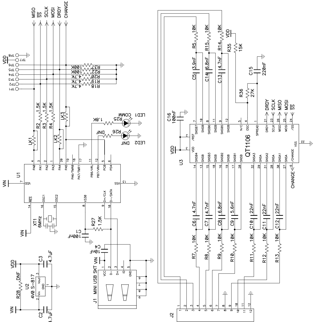
Figure 5: E1106 Circuit Diagram
