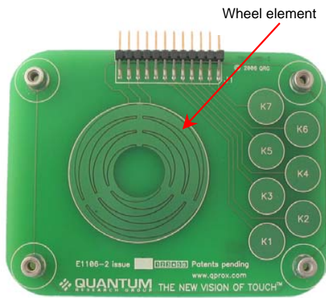
Figure 7: QWheel Assembly Details
