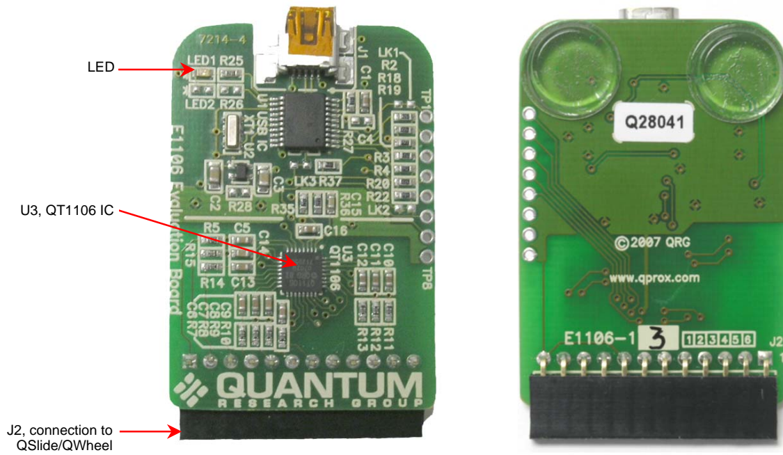
Figure 6: E1106 Control Board Assembly Details
