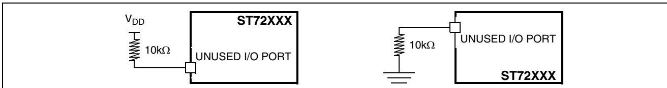
Figure 75 Two typical Applications with unused I/O Pin
