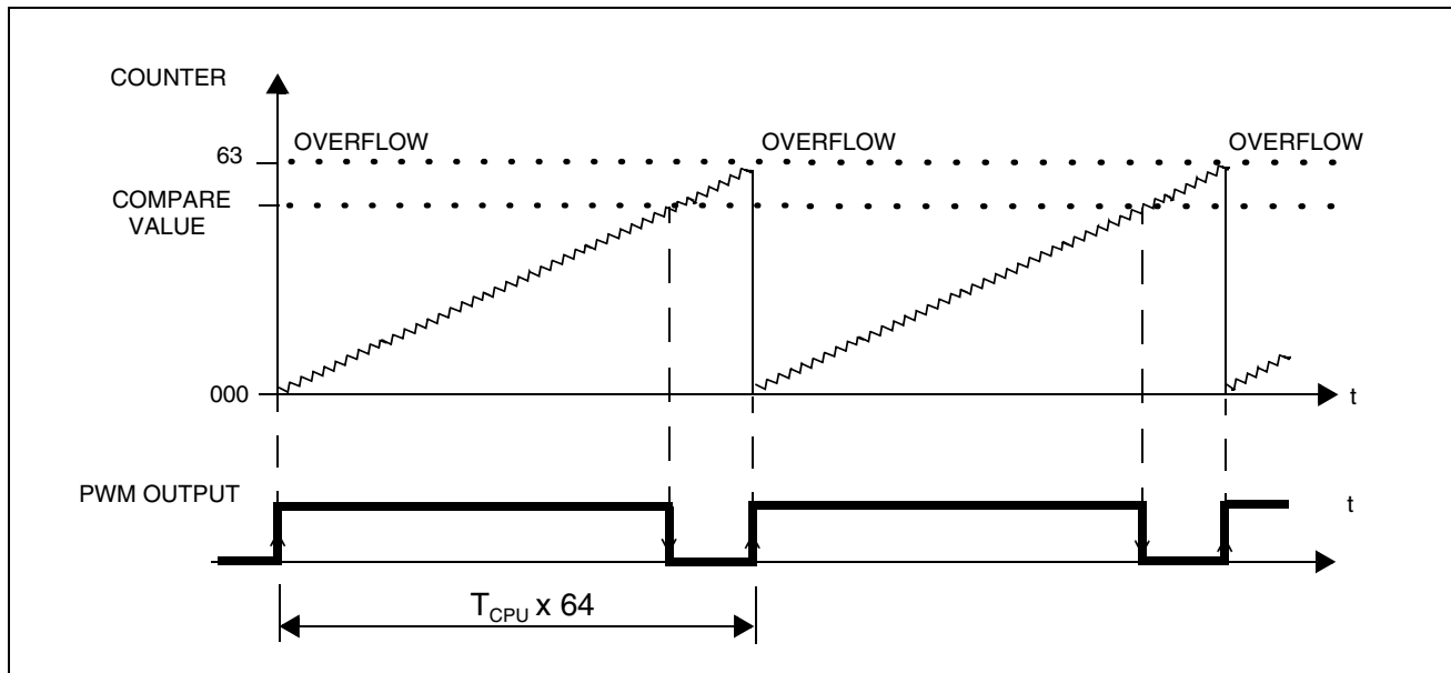
Figure 48. PWM Generation
