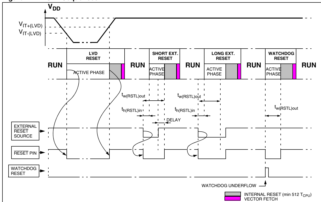
Figure 17. RESET Sequences
