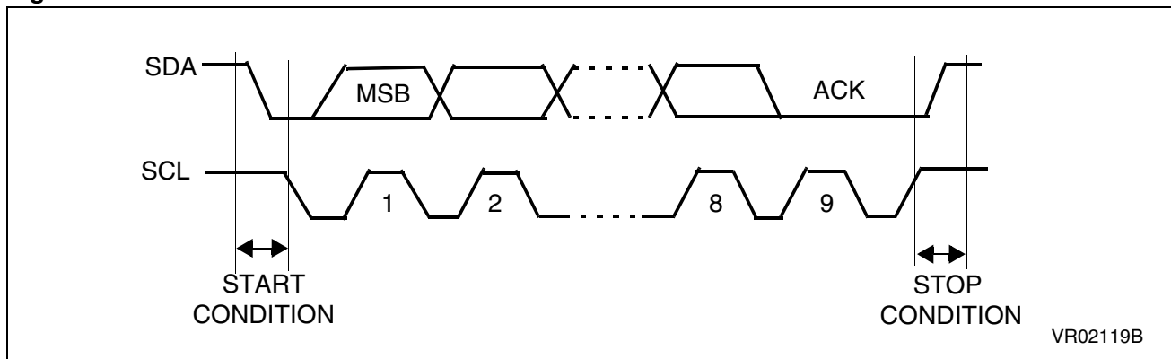
Figure 62. I 2 C BUS Protocol
