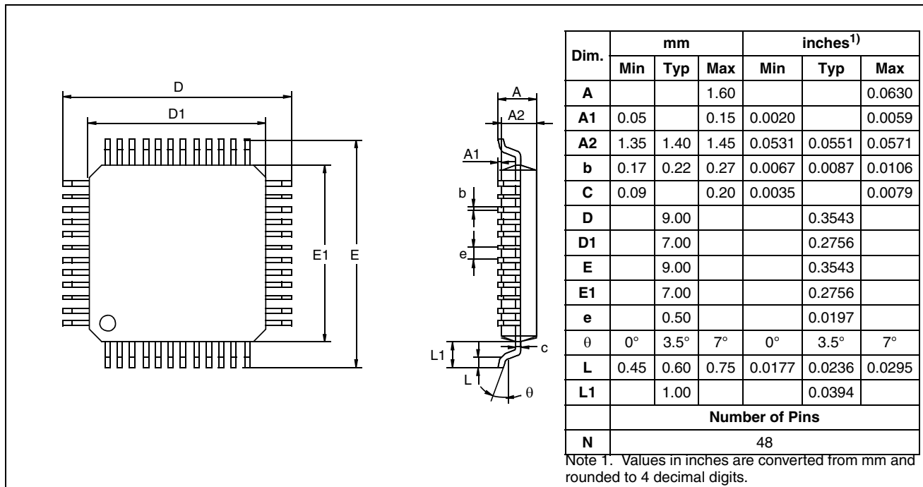
Figure 95. 48-Pin Low profile Quad Flat Package
