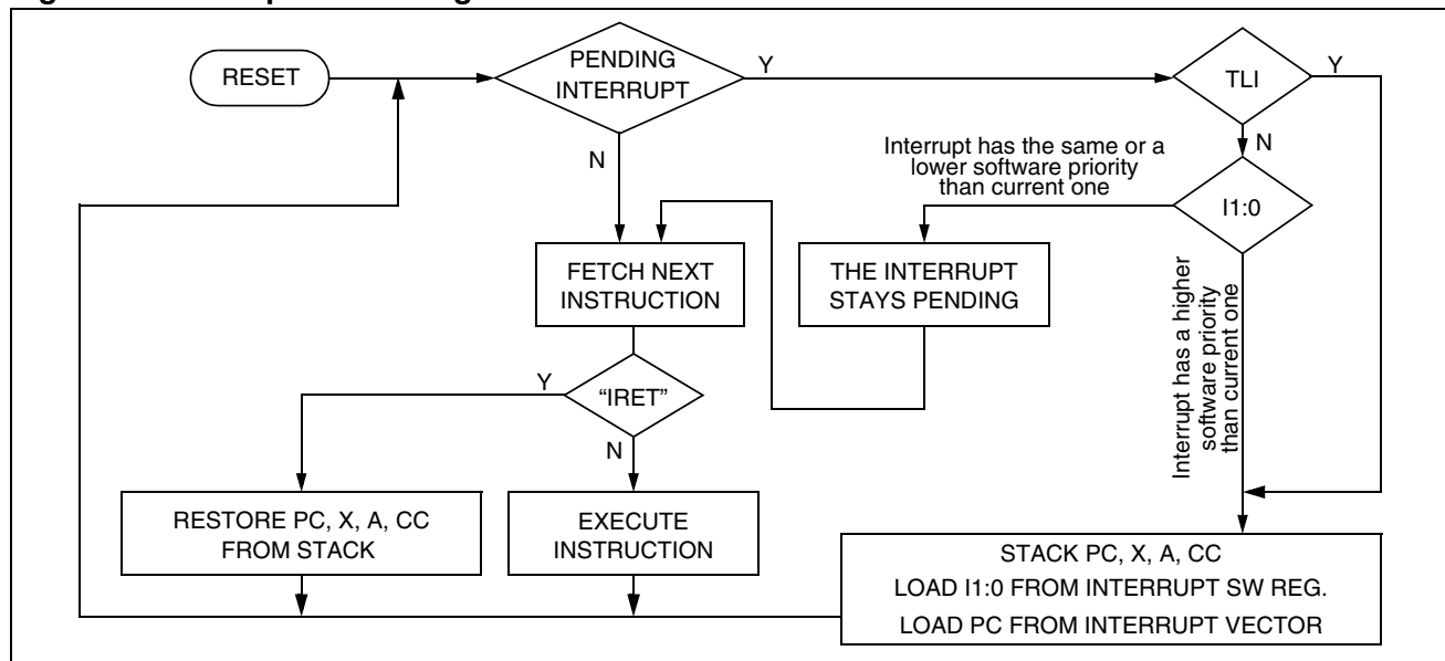
Figure 25. Interrupt Processing Flowchart
