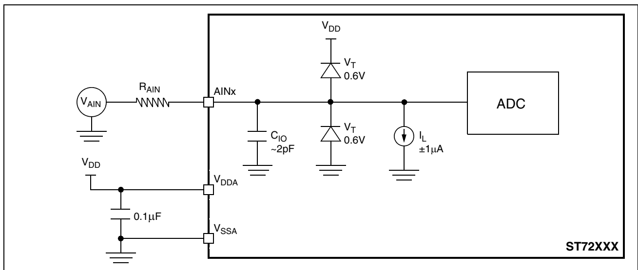
Figure 93. Typical Application with ADC
