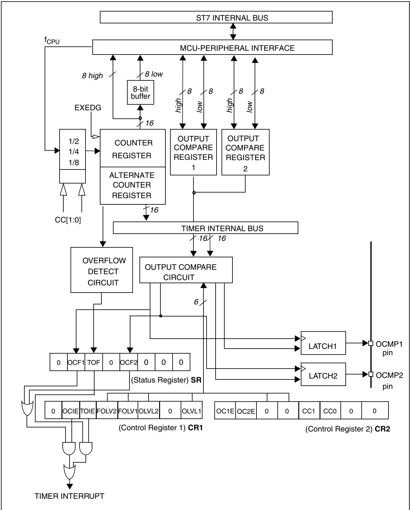
Figure 41. Timer Block Diagram
