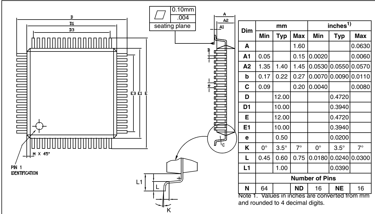
Figure 96. 64-Pin 10 x 10 Low profile Quad Flat Package
