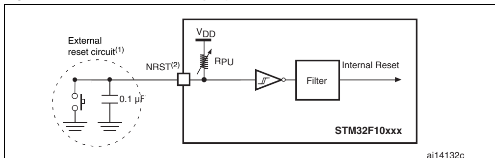
Figure 21. Recommended NRST pin protection
