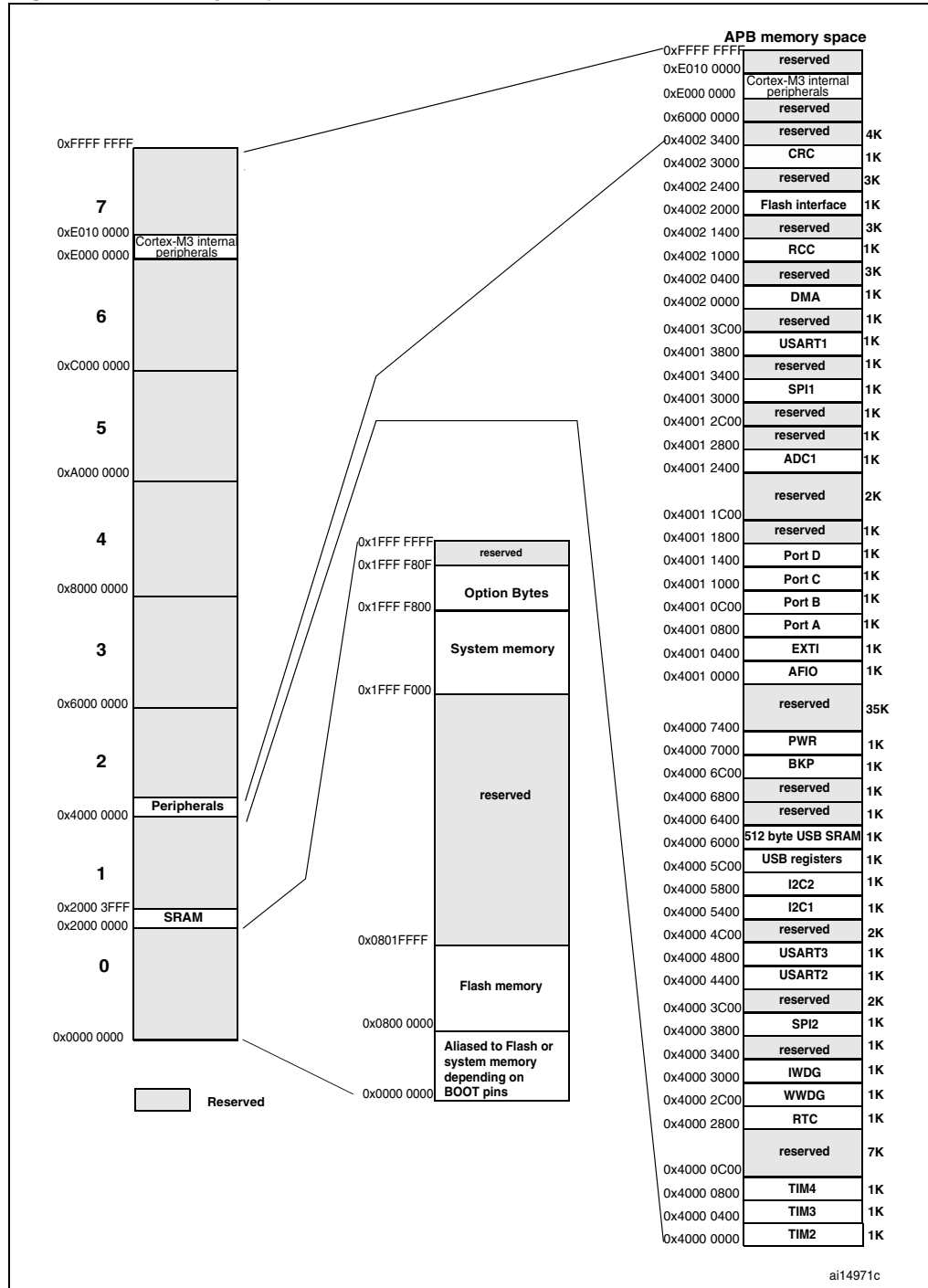
Figure 5. Memory map
