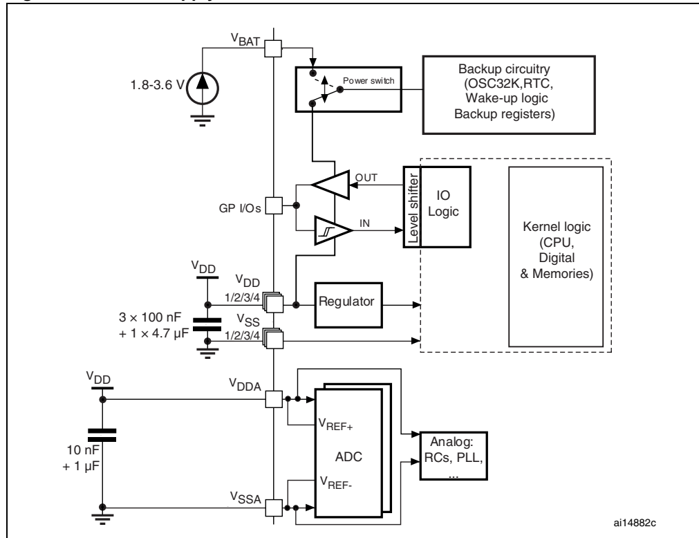
Figure 8. Power supply scheme
