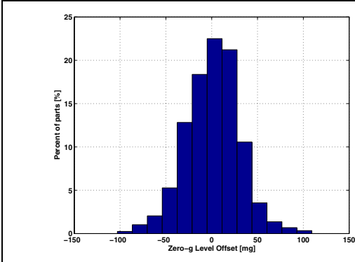
Figure 16. Z axis 0-g level at 2.5V
